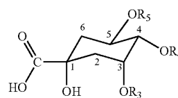
Quinic Acid: R 3 =R 4 =R 5 =H
