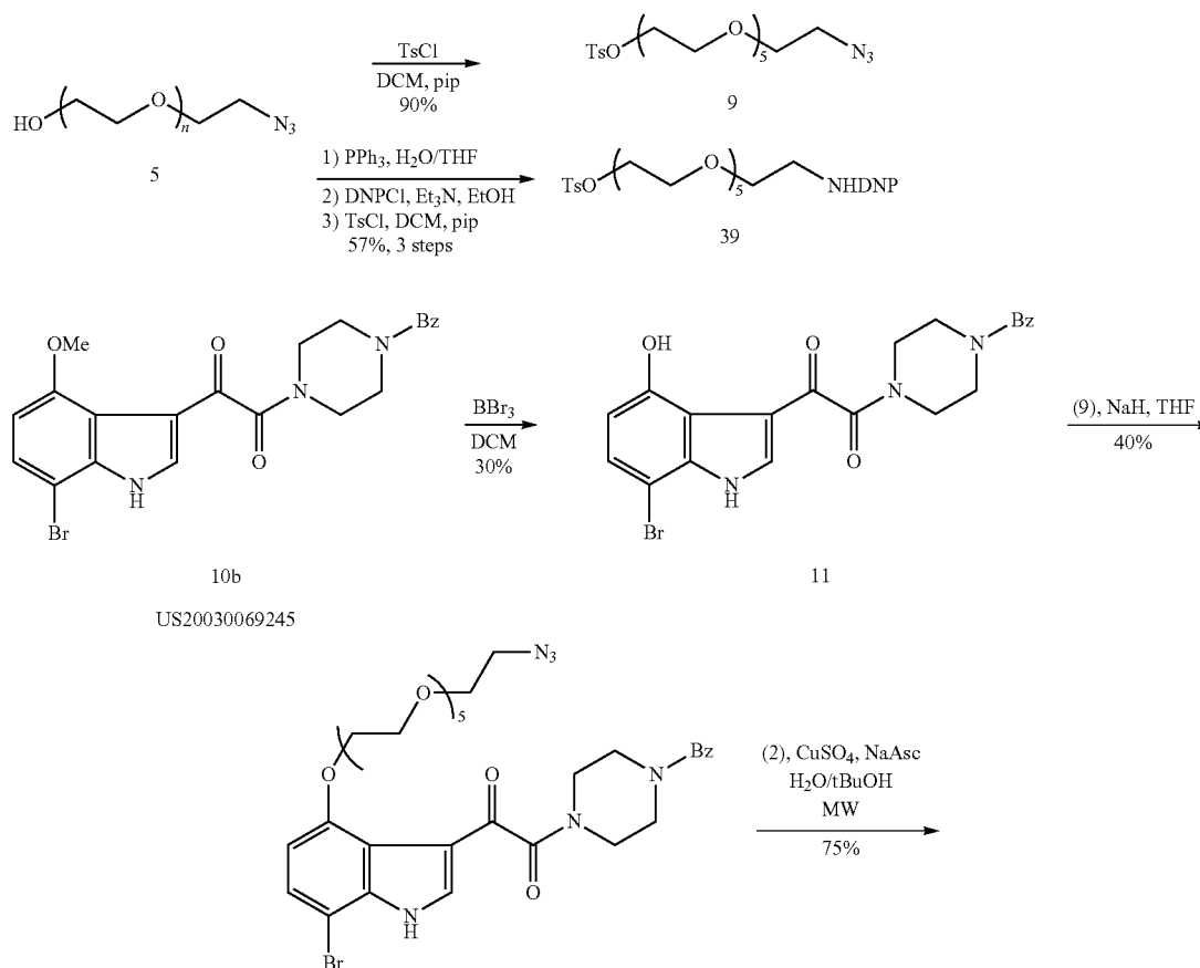
Supplementary Scheme 4. Representative Synthesis of ARM-H type (14) and type (28) molecules
