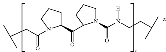
polyproline linker
