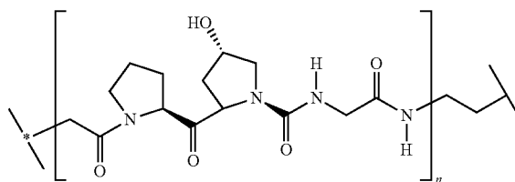
collagen linker
