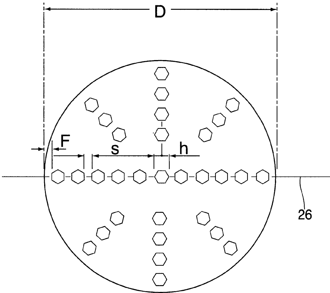
SECTION C-C
