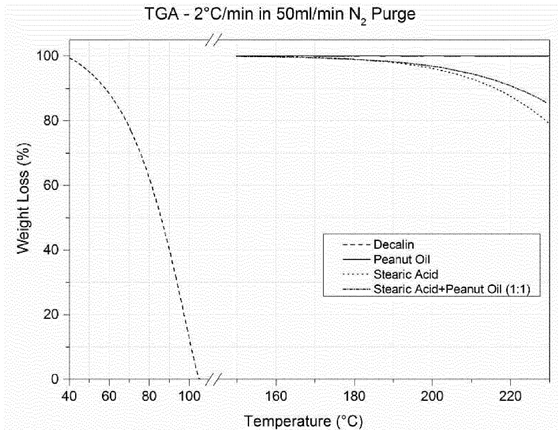
Figure 1 – TGA curves
