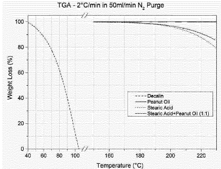
Figure 1 – TGA curves
