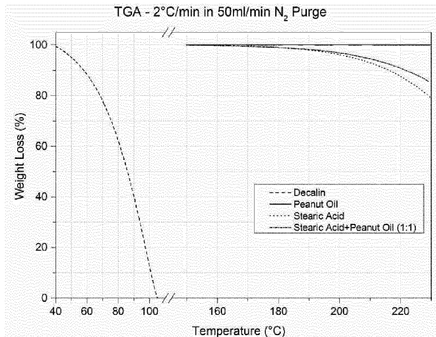
Figure 1 – TGA curves
