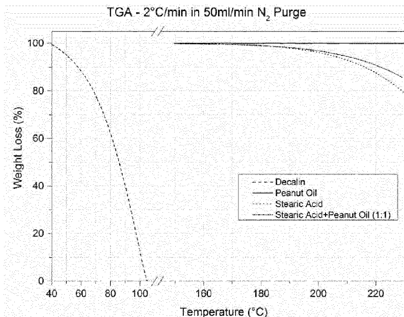
Figure 1 – TGA curves
