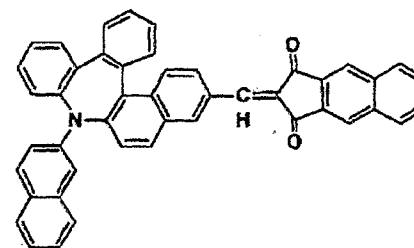
COMPOUND 22
