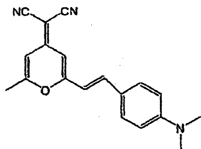
COMPOUND 9
