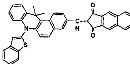
COMPOUND 24
