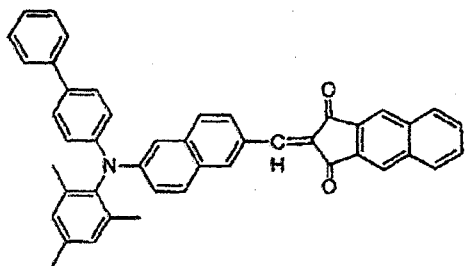
COMPOUND 19
