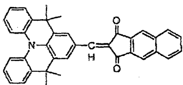
COMPOUND 23
