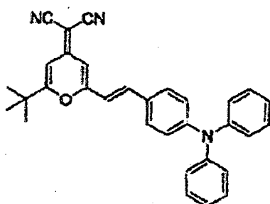
COMPOUND 13
