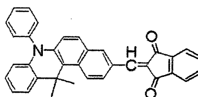
COMPOUND 8
