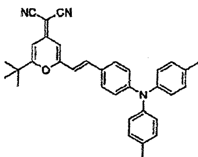
COMPOUND 13
