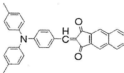
COMPOUND 4
