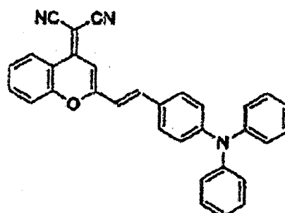
COMPOUND 14
