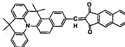
COMPOUND 22
