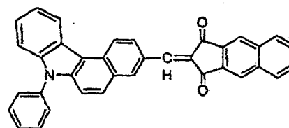
COMPOUND 18
