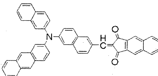
COMPOUND 6
