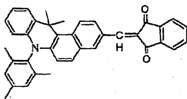
COMPOUND 21
