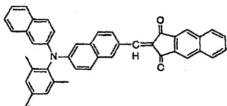
COMPOUND 15
