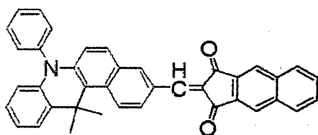
COMPOUND 7
