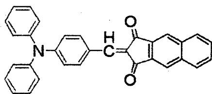
COMPOUND 3
