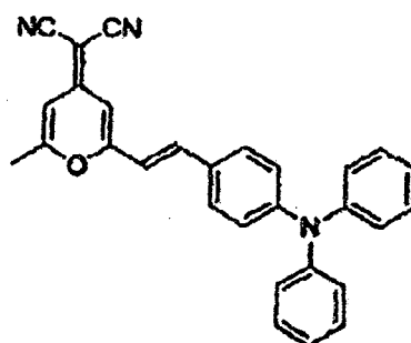
COMPOUND 12
