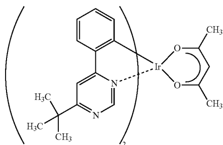
[Ir(tBuppm) 2 (acac)]
