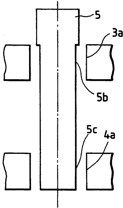
FIG. 15 (PRIOR ART)
