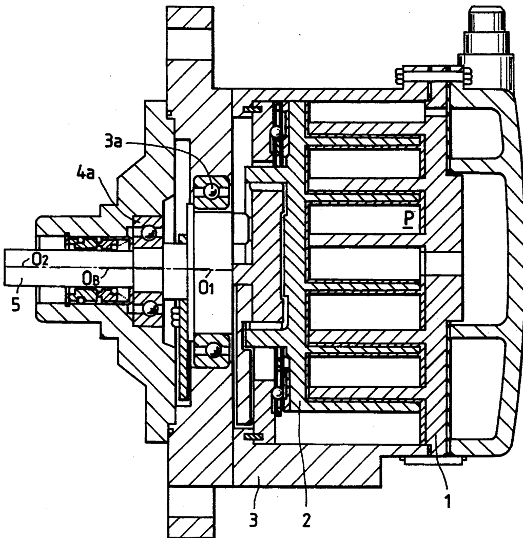
FIG. 17 (PRIOR ART)
