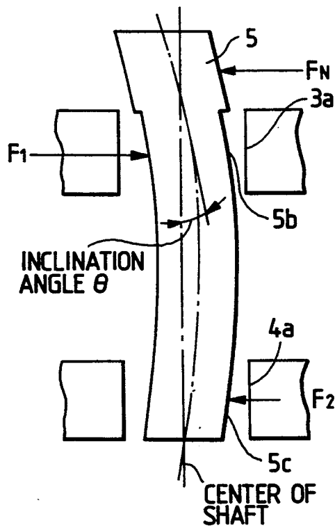
FIG. 16 (PRIOR ART)
