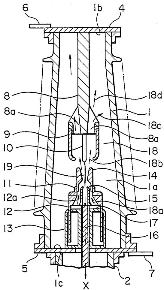
FIG. 2 PRIOR ART
