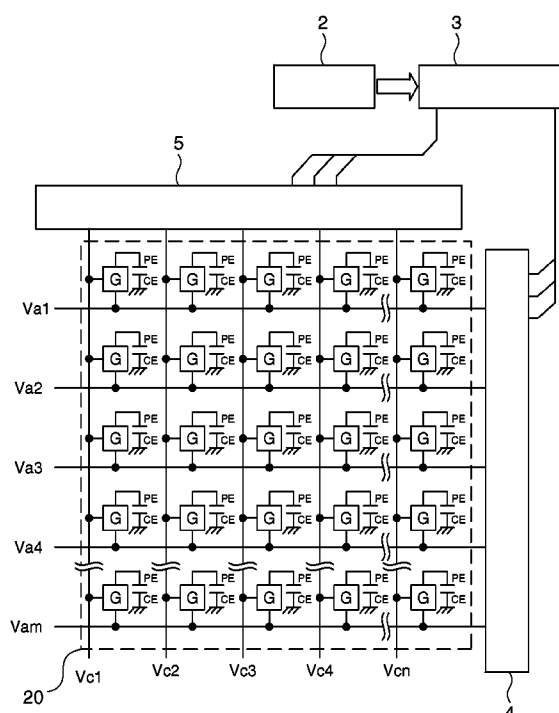
10 : ELECTROPHORETIC DISPLAY DEVICE
