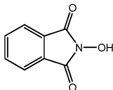
1-hydroxybenzotriazole
