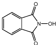
N-hydroxyphthalimide
