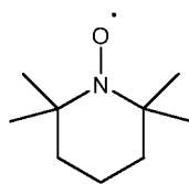
2,2,6,6-tetramethyl-1-piperidinyloxy (TEMPO)
