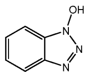
1-hydroxybenzotriazole
