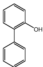
2-hydroxybiphenyl
