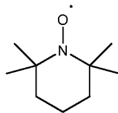
2,2,6,6-tetramethyl-1-piperidinyloxy (TEMPO)
