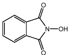
N-hydroxyphthaleimide
