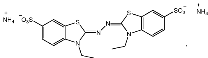
2,2'-azine-bis(3-ethylbenzothiazoline-6-sulfonic acid) (ABTS)
