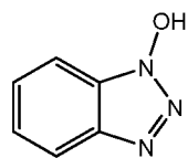
1-hydroxybenzotriazole
