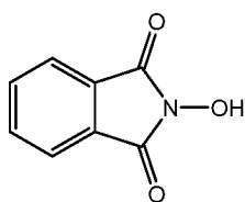
N-hydroxyphthalimide
