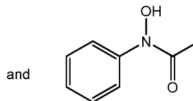
N-hydroxyacetanilide
