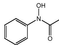
N-hydroxyacetanilide
