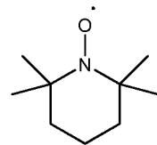
2,2,6,6-tetramethyl-1-piperadinyloxy (TEMPO)
