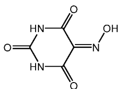
violuric acid
