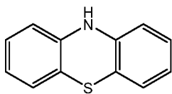
10-H-phenothiazine
