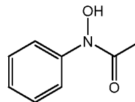
N-hydroxyacetanilide
