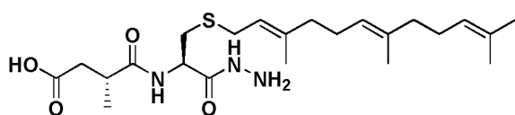
N-34a [3-me regioisomer R-R enantiomer] enantiomer]
