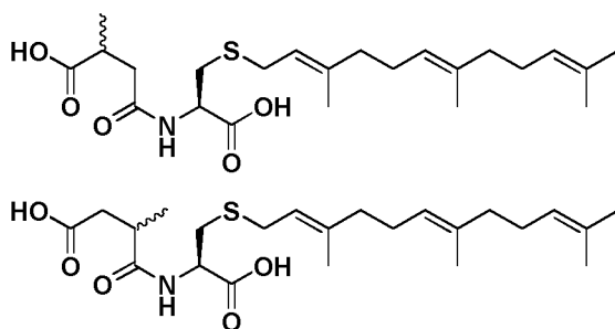
N-22 [3-me regioisomer racemate]
