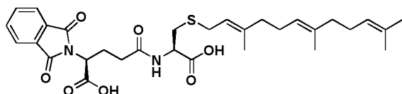
C-1 [(R)-(R) isomer]
