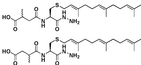
N-34 [3-me regioisomer racemate]
