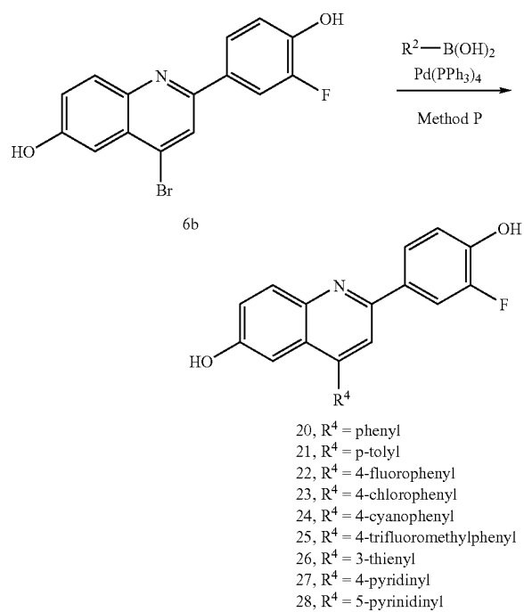
Scheme 7
