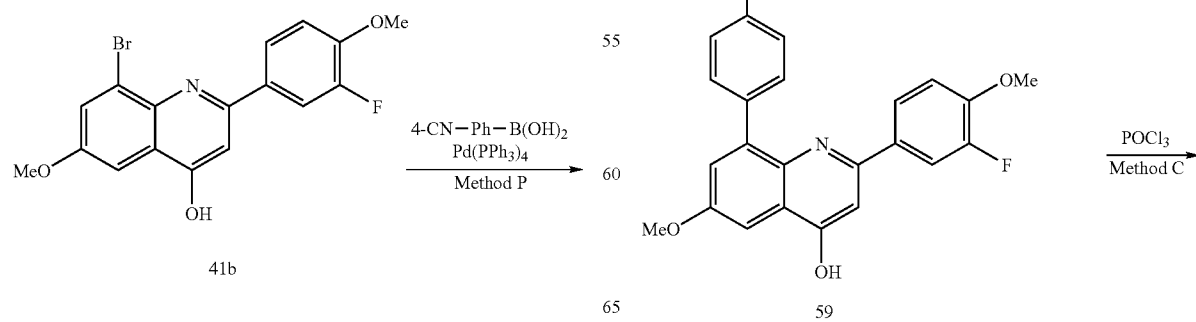
Scheme 16
