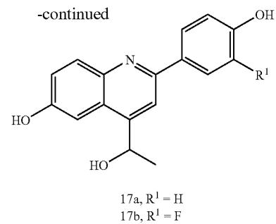
Scheme 6
