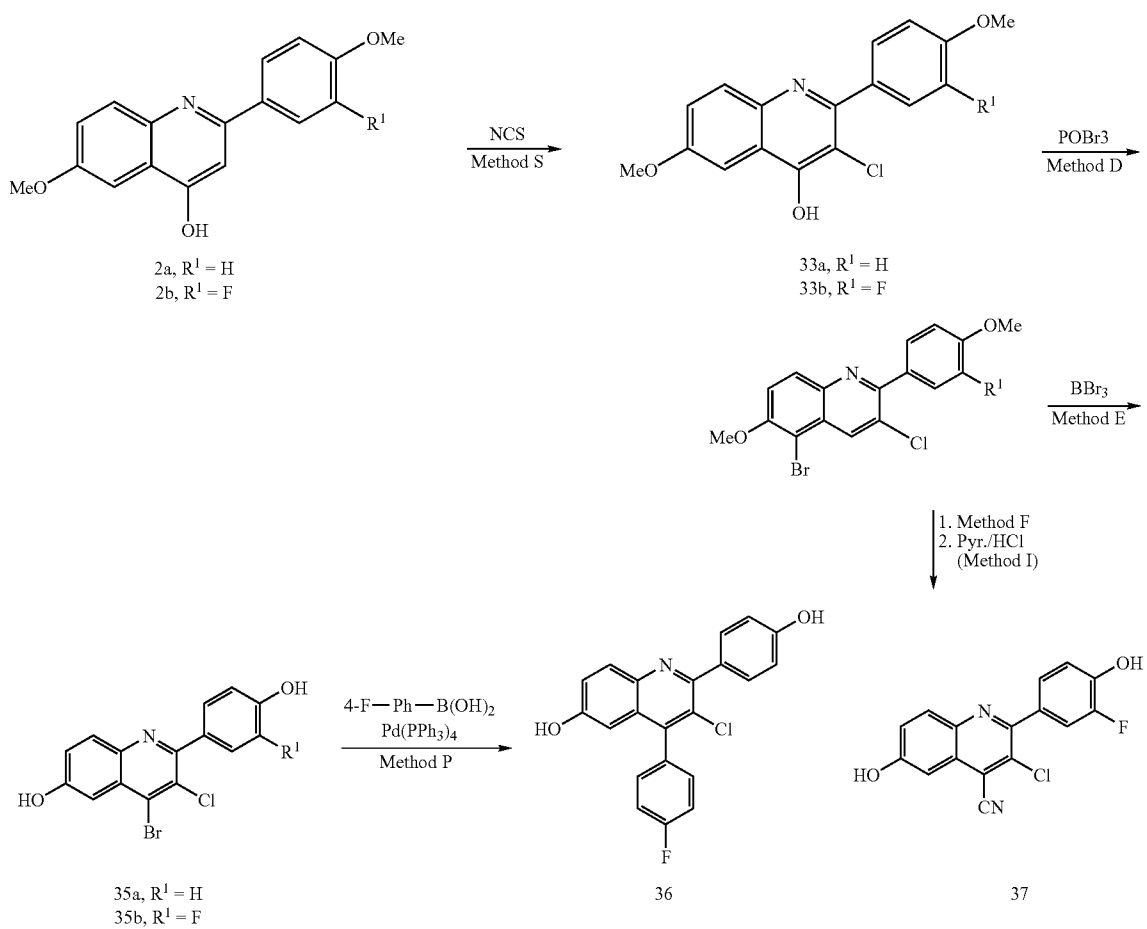
Scheme 9
