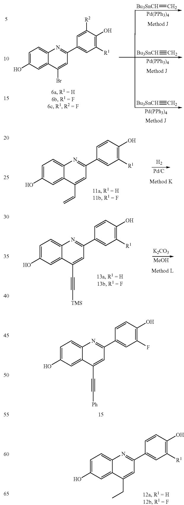
Scheme 4
