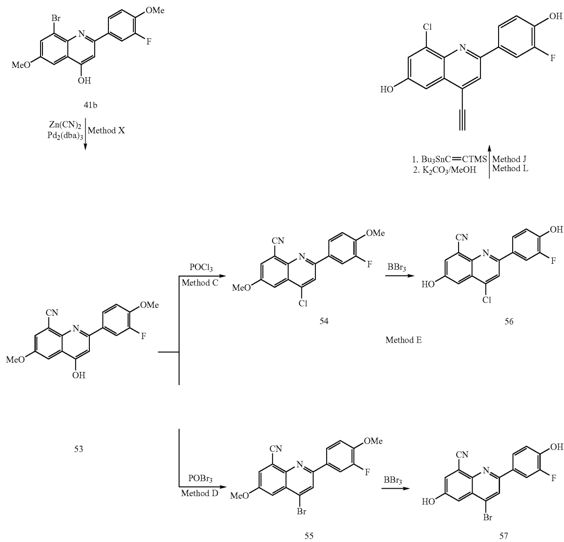
Scheme 15
