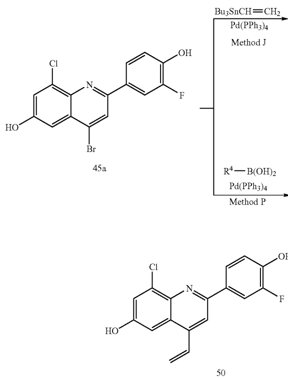
Scheme 14
