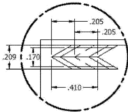
DETAIL E
