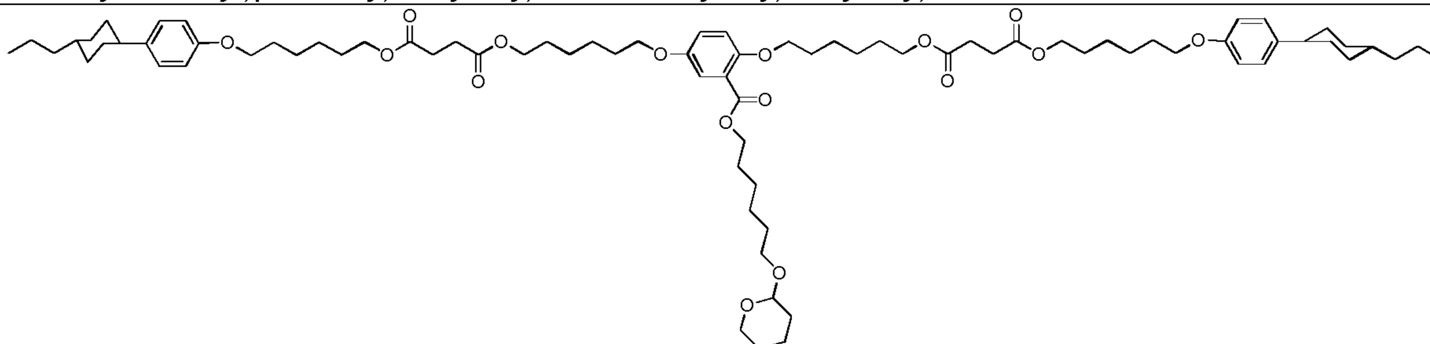
2,5-bis{6-(4-(6-(4-(trans-4-propylcyclohexyl)phenoxy)hexyloxy)-4-oxobutoyloxy)hexyloxy}-1-(6-(tetrahydro-2H-pyran-2-yloxy)hexyl)benzoate
