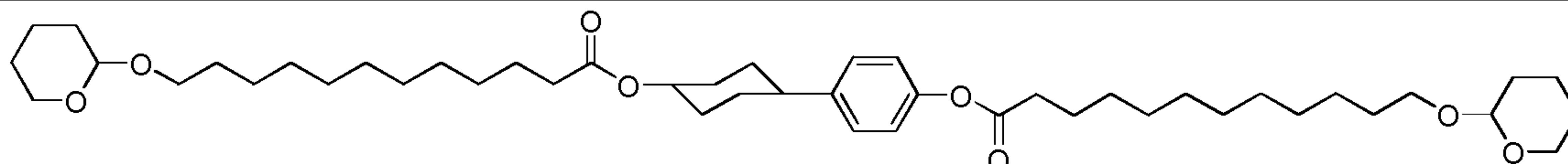
2-(6-(trans-4-(4-(12-(tetrahydro-2H-pyran-2-yloxy)dodecanoyloxy)cyclohexyl)phenoxy)-12-oxododecanoyl)tetrahydro-2H-pyran
