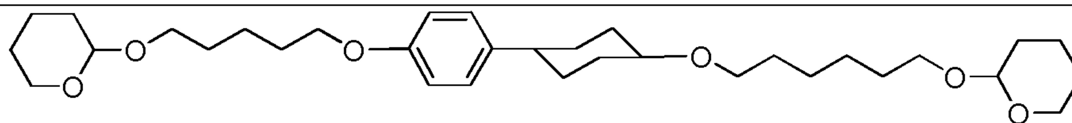
2-(5-(trans-4-(4-(6-(tetrahydro-2H-pyran-2-yloxy)hexyloxy)cyclohexyl)benzyloxy)pentyloxy)tetrahydro-2H-pyran
