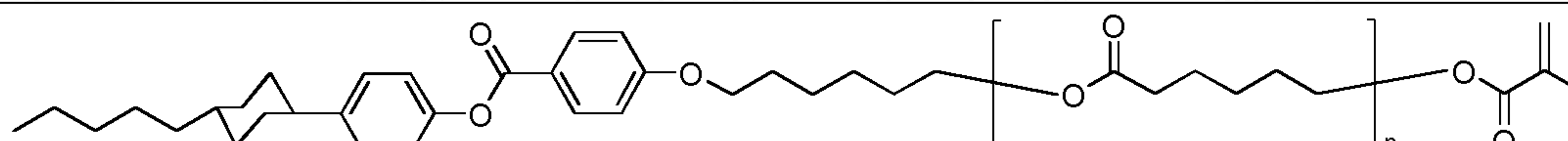
1-(5-(5-(5-(5-(6-(4-(4-(trans-4-pentylcyclohexyl)phenoxy)carbonyl)phenoxy)hexyloxy)-5-oxopentyloxy)-5-oxopentyloxy)-5-oxopentyloxy)-2-methylprop-2-en-1-one
