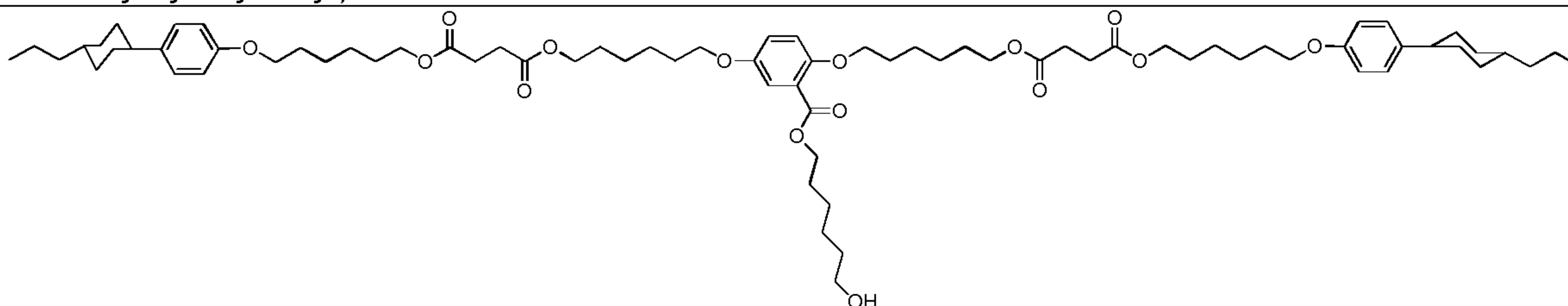
2,5-bis{6-(4-(6-(4-(trans-4-propylcyclohexyl)phenoxy)hexyloxy)-4-oxobutoyloxy)hexyloxy}-1-(6-hydroxyhexyl)benzoate
