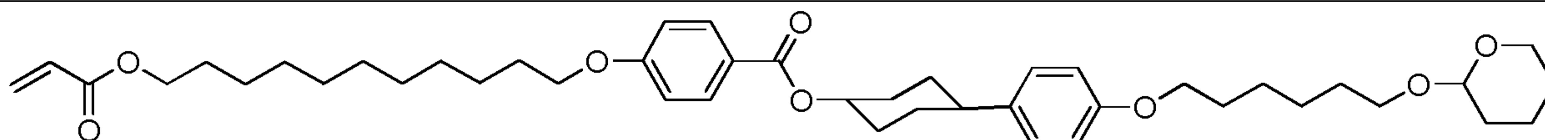
1-(11-(4-(trans-4-(4-(6-(1-(tetrahydro-2H-pyran-2-yloxy)hexyloxy)phenyl)cyclohexyloxycarbonyl)phenoxy)undecanoyloxy)prop-2-en-1-one
