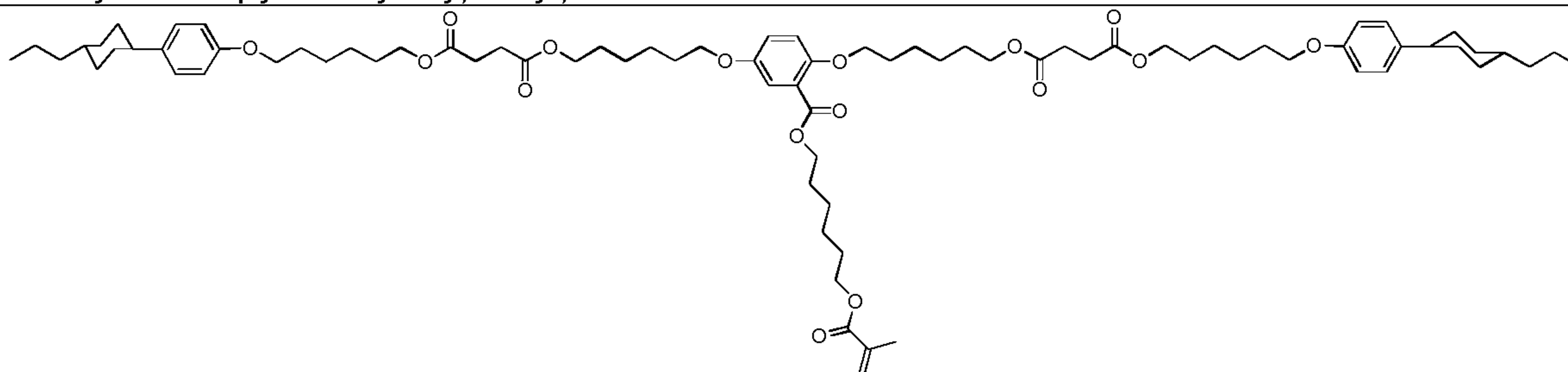
2,5-bis{6-(4-(6-(4-(trans-4-propylcyclohexyl)phenoxy)hexyloxy)-4-oxobutoyloxy)hexyloxy}-1-(6-methacryloyloxyhexyl)benzoate
