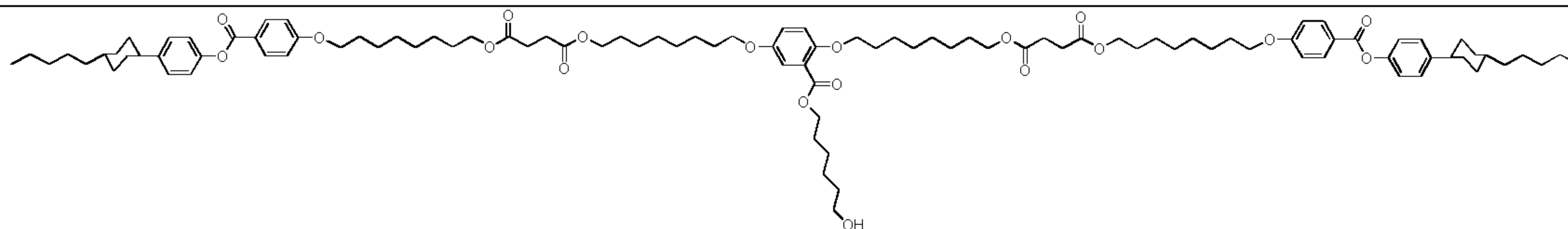
6-hydroxyhexyl 2,5-bis(8-(3-(8-(4-(4-(trans-4-pentylcyclohexyl)phenoxy)carbonyl)phenoxy)octyloxy)-4-oxobutoyloxy)octyloxy)benzoate
