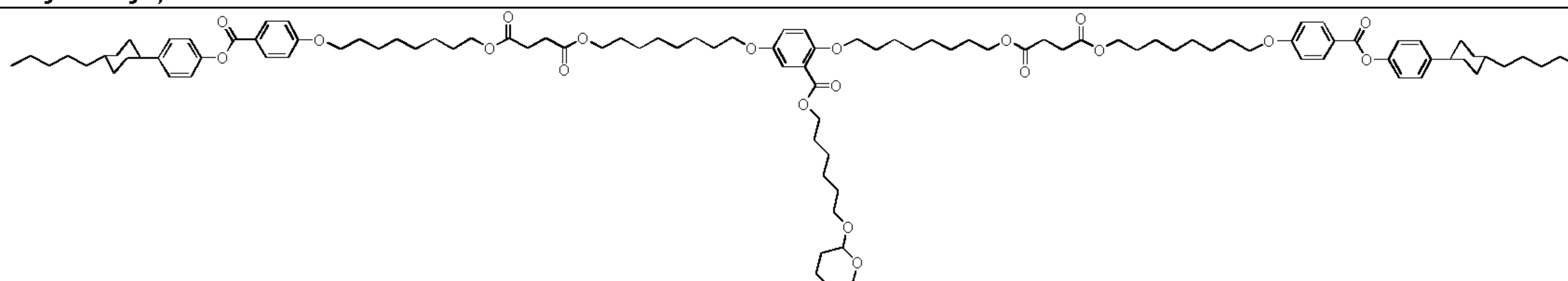
6-(tetrahydro-2H-pyran-2-yloxy)hexyl 2,5-bis(8-(3-(8-(4-(4-(trans-4-pentylcyclohexyl)phenoxy)octyloxy)-4-oxobutoyloxy)octyloxy)benzoate
