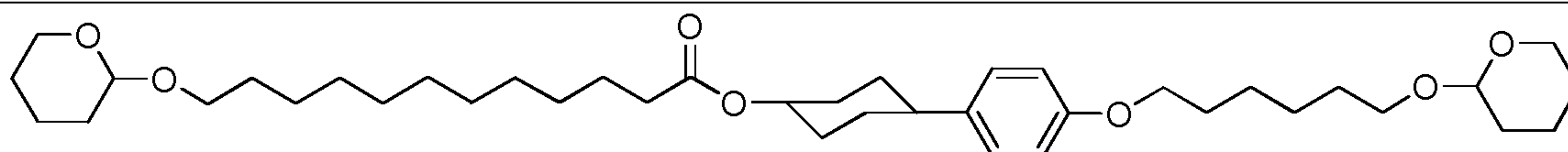
2-(6-(4-(trans-4-(12-(1-tetrahydro-2H-pyran-2-yloxy)dodecanoyloxy)cyclohexyl)phenoxy)hexyloxy)tetrahydro-2H-pyran
