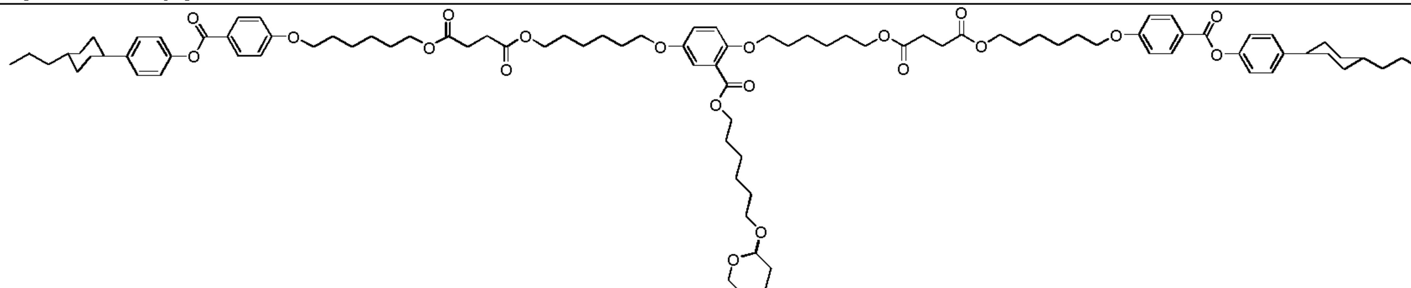
6-(tetrahydro-2H-pyran-2-yloxy)hexyl 2,5-bis(6-(3-(6-(4-(4-(trans-4-pentylcyclohexyl)phenoxy)hexyloxy)-4-oxobutoyloxy)hexyloxy)benzoate
