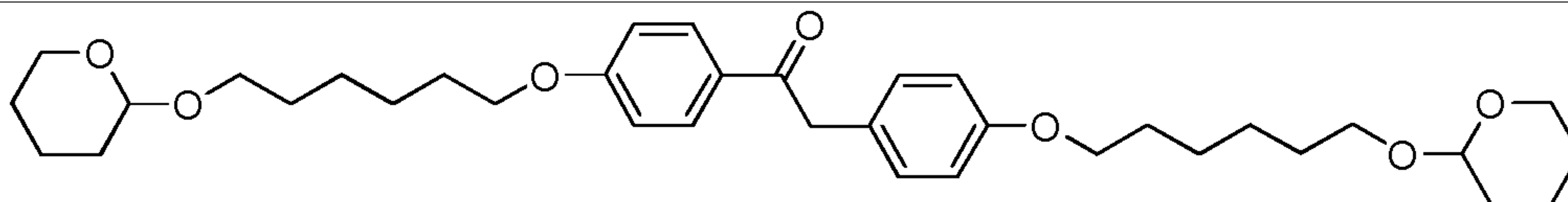
1,2-bis(4-(6-(tetrahydro-2H-pyran-2-yloxy)hexyloxy)phenyl)ethanone
