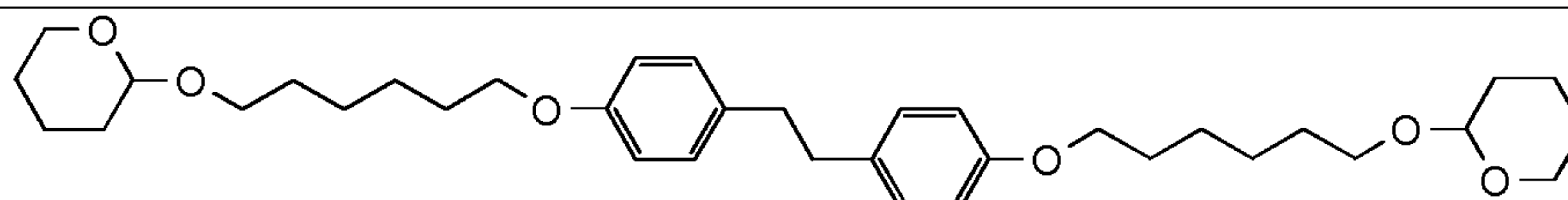
1,2-bis(4-(6-(tetrahydro-2H-pyran-2-yloxy)hexyloxy)phenyl)ethane
