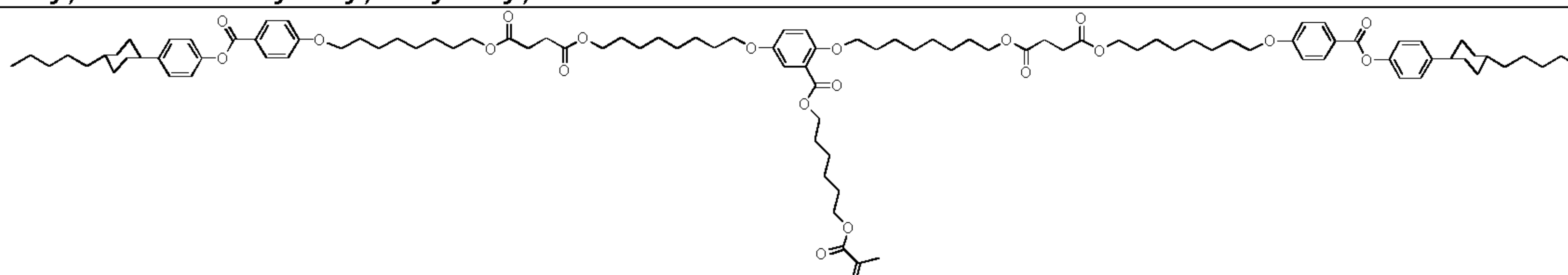
6-methacryloyloxyhexyl 2,5-bis(8-(3-(8-(4-(4-(trans-4-pentylcyclohexyl)phenoxy)carbonyl)phenoxy)octyloxy)-4-oxobutoyloxy)octyloxy)benzoate
