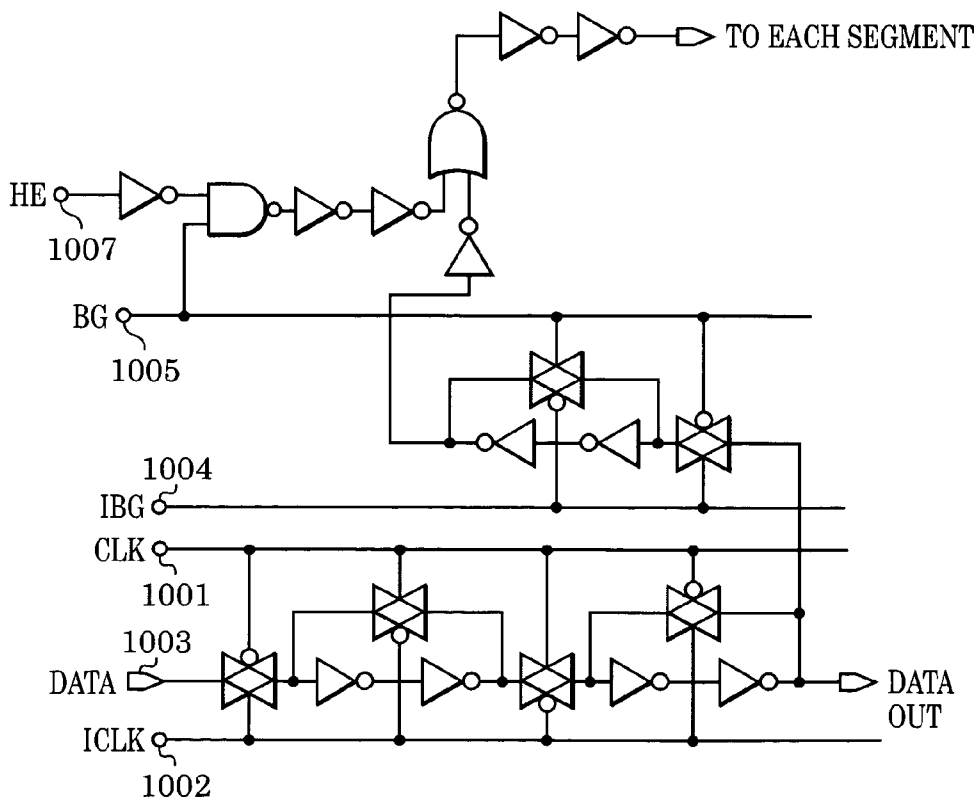
FIG. 13 (PRIOR ART)
