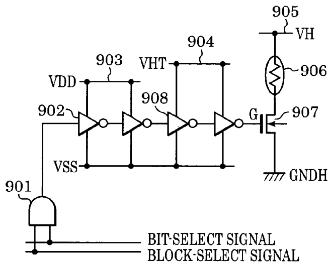
FIG. 12 (PRIOR ART)
