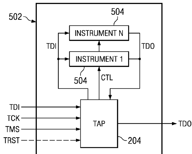
FIG. 6 (PRIOR ART)
