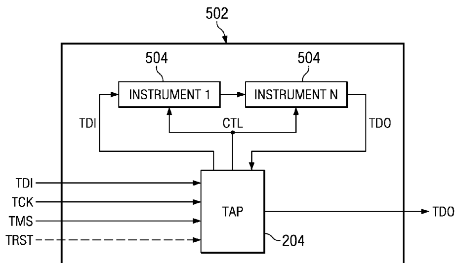
FIG. 7 (PRIOR ART)
