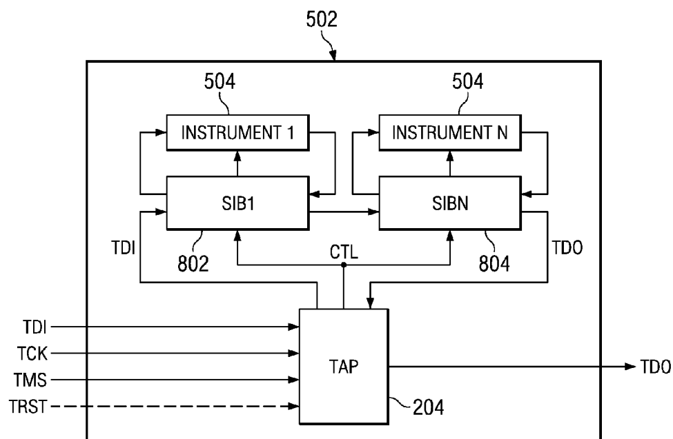
FIG. 8 (PRIOR ART)
