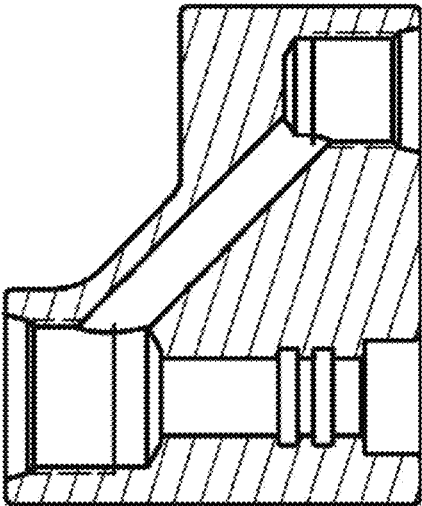
SECTION A-A SCALE 1
