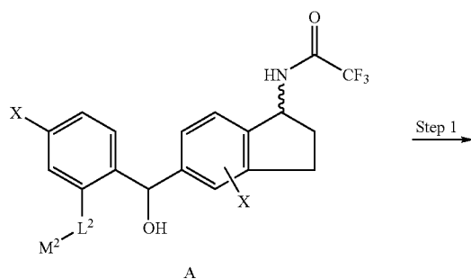
General Scheme V Preparation of Phenyl Carbonyl Linked Compounds
