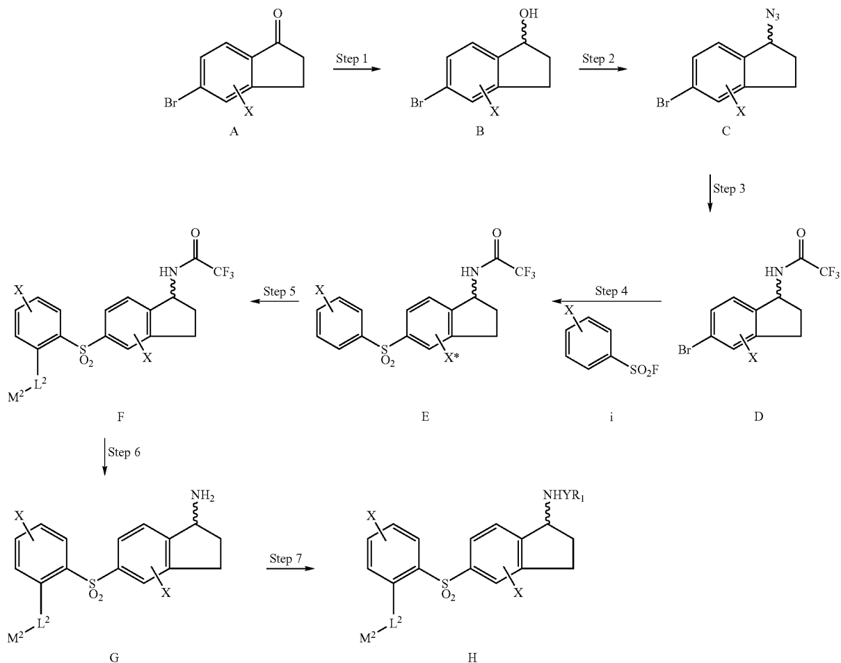
General Scheme I Preparation of Phenyl Compounds
