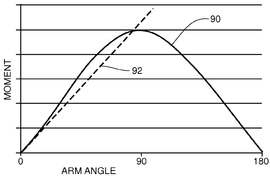
FORCE CURVE FOR ARM
