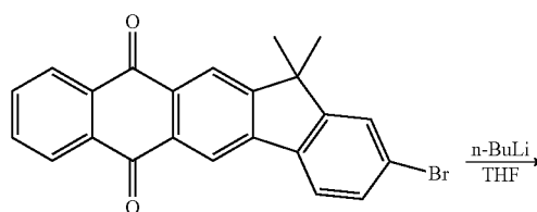
[Reaction Scheme 6]
