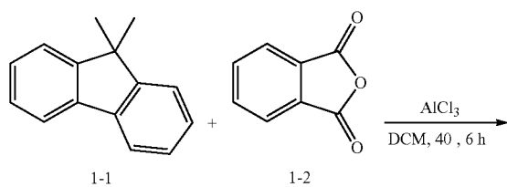
[Reaction Scheme 15]
