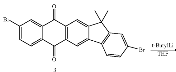
[Reaction Scheme 13]
