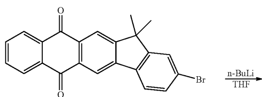
[Reaction Scheme 7]
