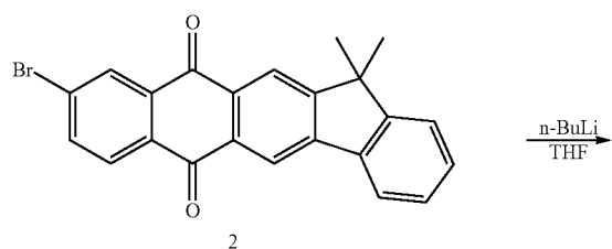
[Reaction Scheme 2]
