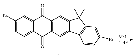
[Reaction Scheme 12]
