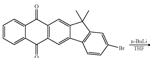
[Reaction Scheme 8]
