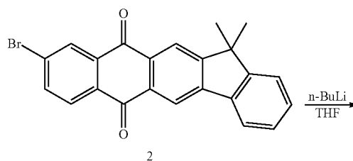
[Reaction Scheme 3]
