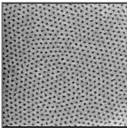
Blend of random copolymer Example 2 and Rexample 4 in 60:40 wt ratio to form contact hole
