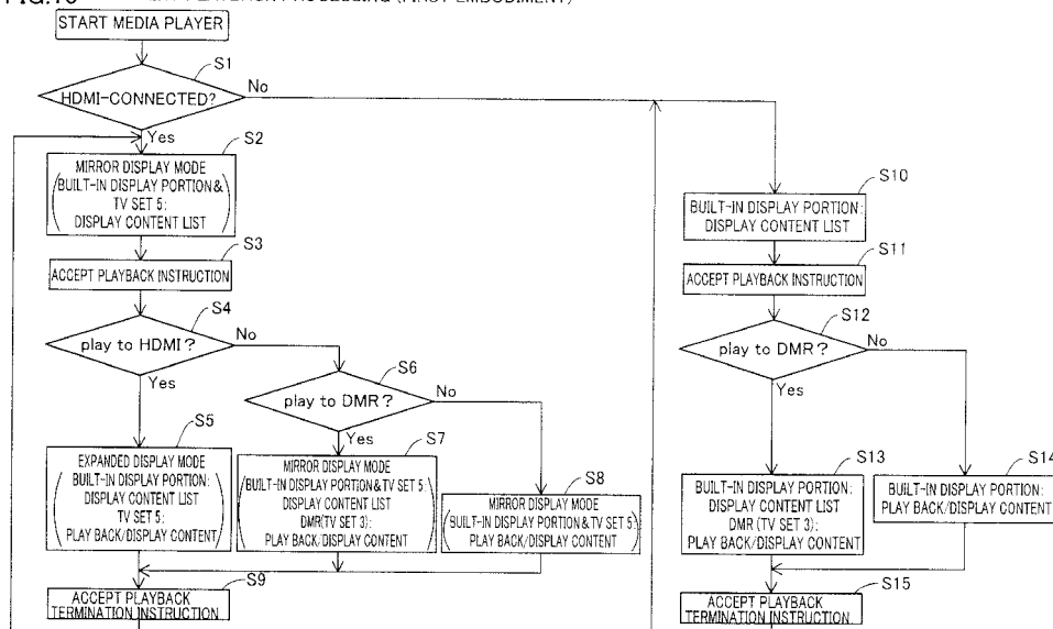
FIG.10 CONTENT PLAYBACK PROCESSING (FIRST EMBODIMENT)
