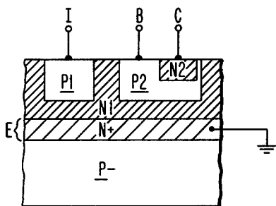
FIG. 1C (PRIOR ART)
