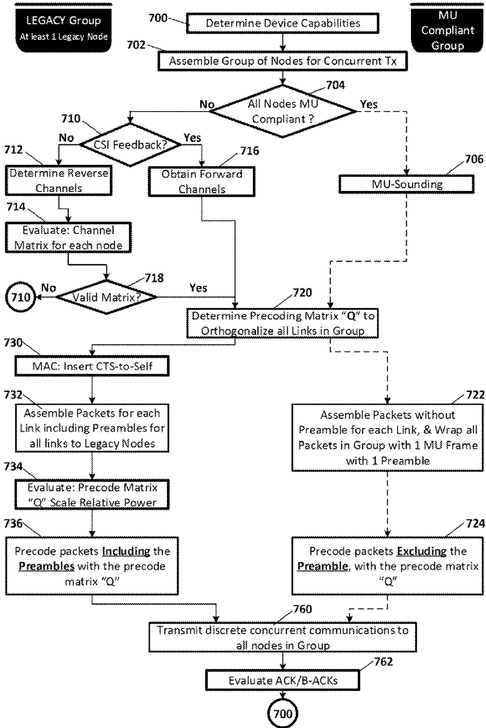
FIG. 7 DUAL MODE CONCURRENT LINK OPERATION
