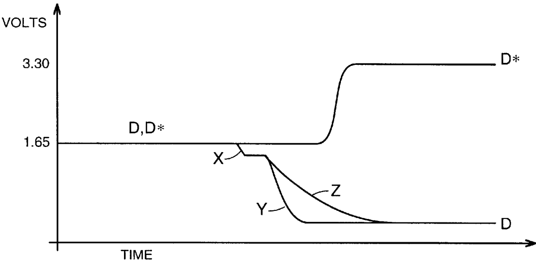
FIG. 2 (PRIOR ART)
