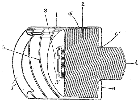
Sectional view
