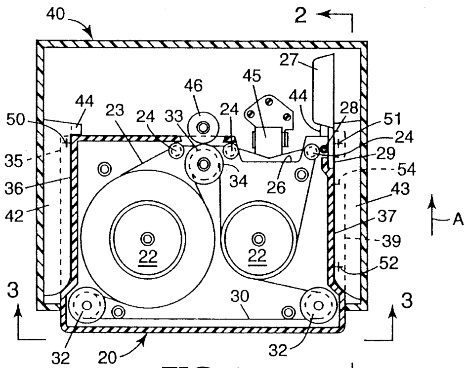
FIG. 1 (PRIOR ART)
