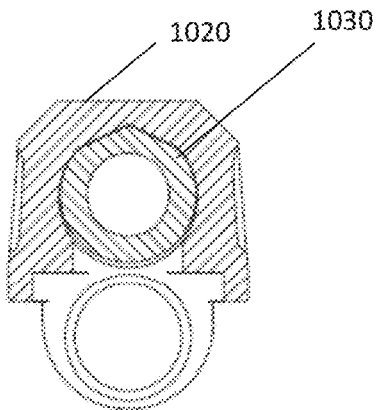
SECTION AW-AW
