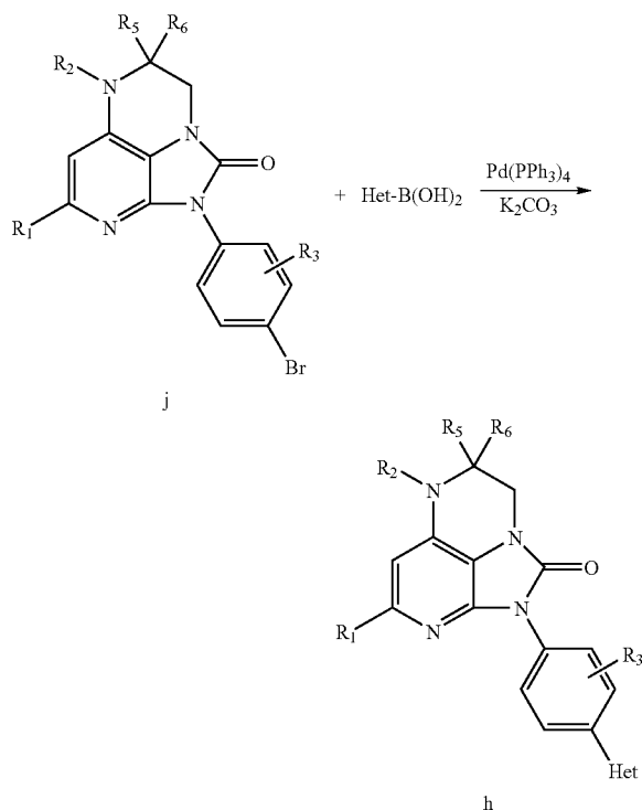
Reaction Scheme 4
