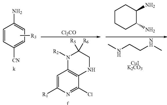
Reaction Scheme 6
