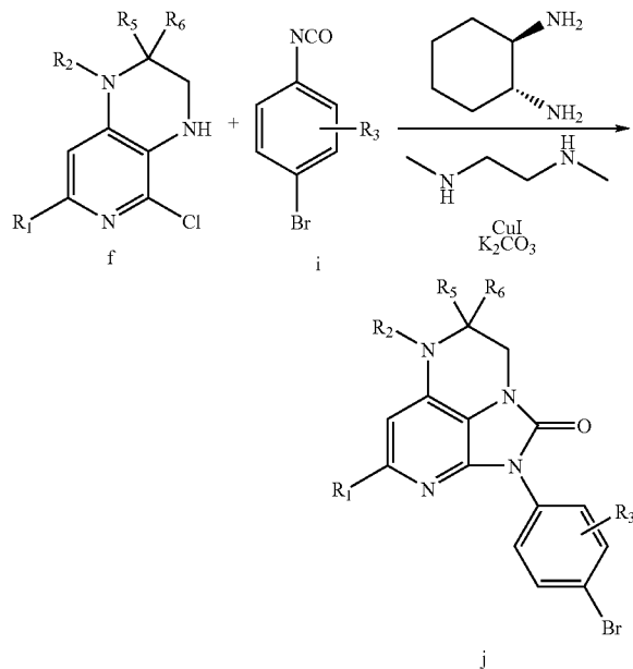
Reaction Scheme 3
