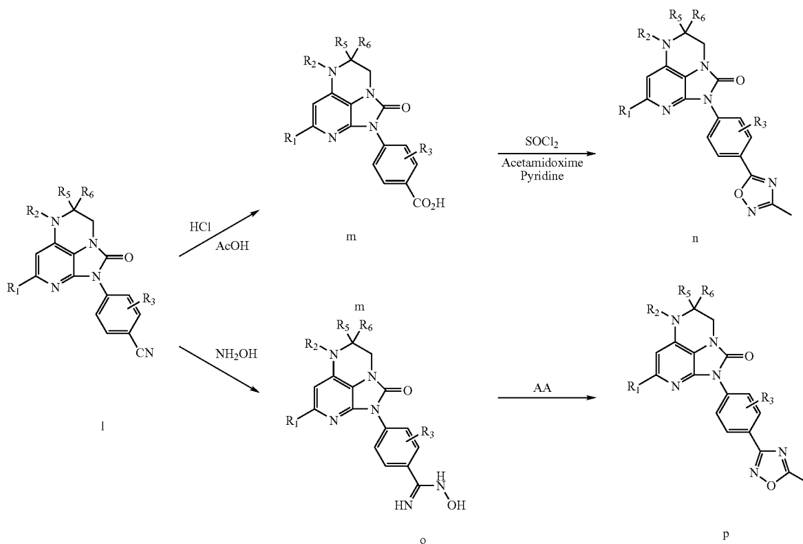
Reaction Scheme 7
