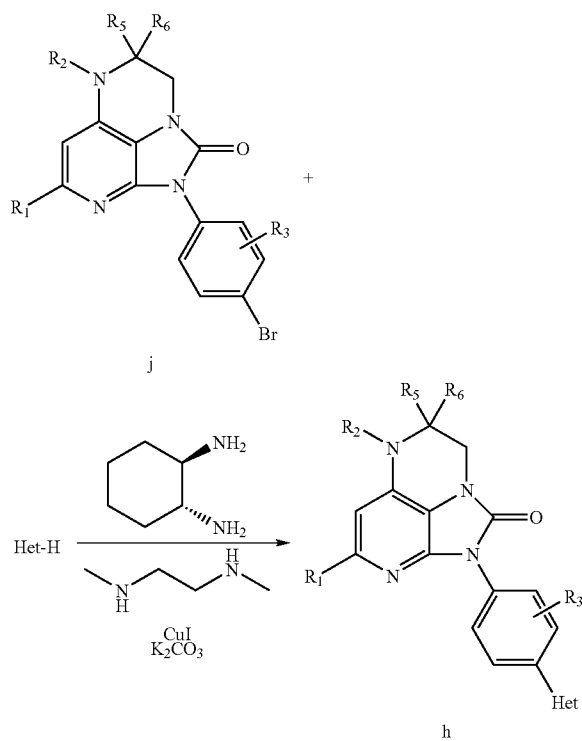
Reaction Scheme 5
