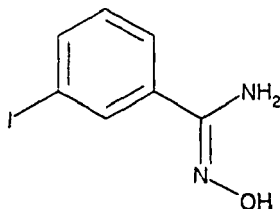
3-Iodophenylamidoxime
