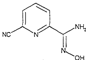
6-Cyano-pyrid-2-yl-amidoxime
