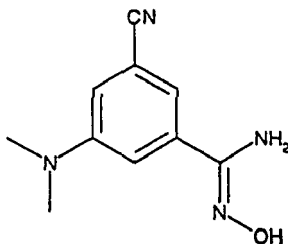
3-Cyano-5-dimethylaminophenylamidoxime
