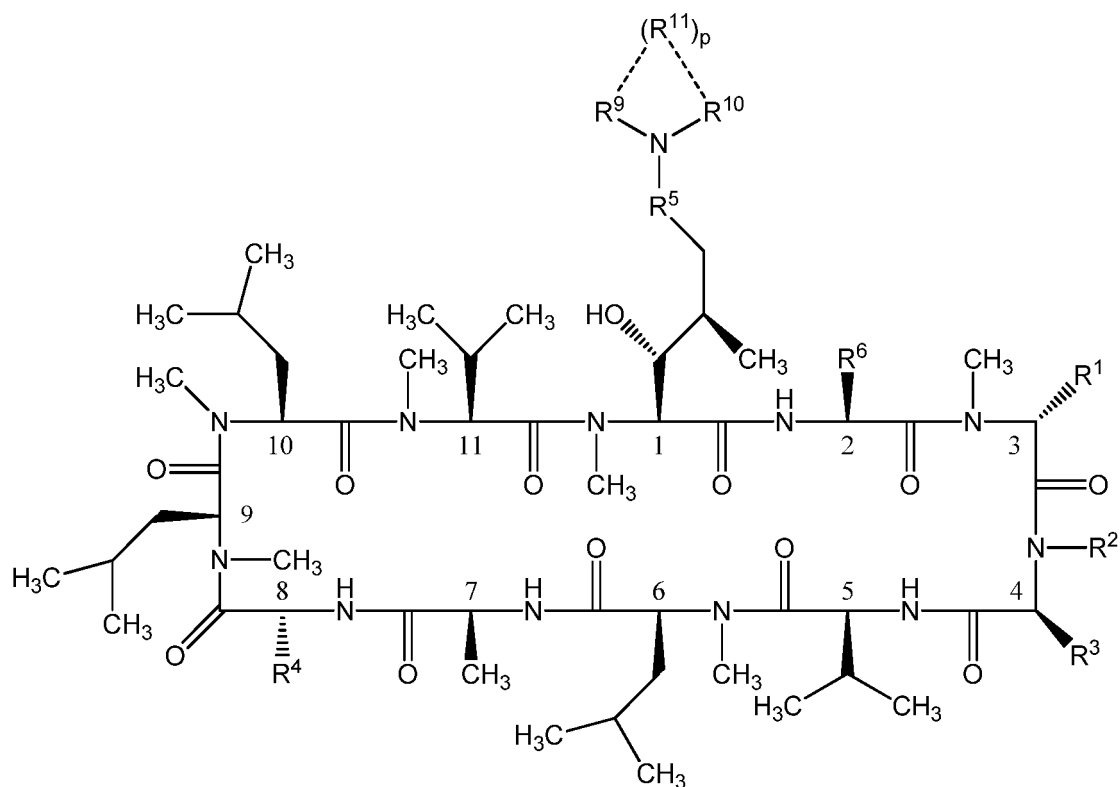
Formula I
