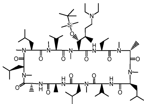
Intermediate 51
