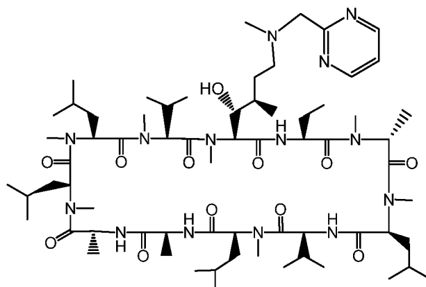
Compound DG
