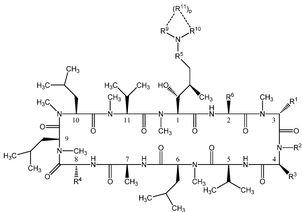
Formula I
