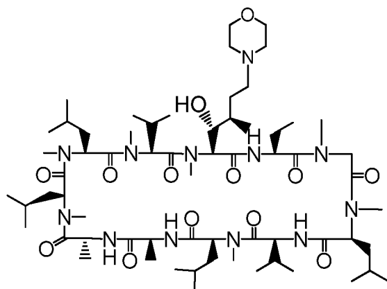
Compound A
