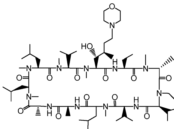
Compound EJ
