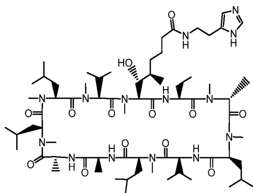
Compound Y
