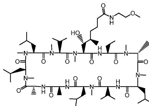
Compound ZY
