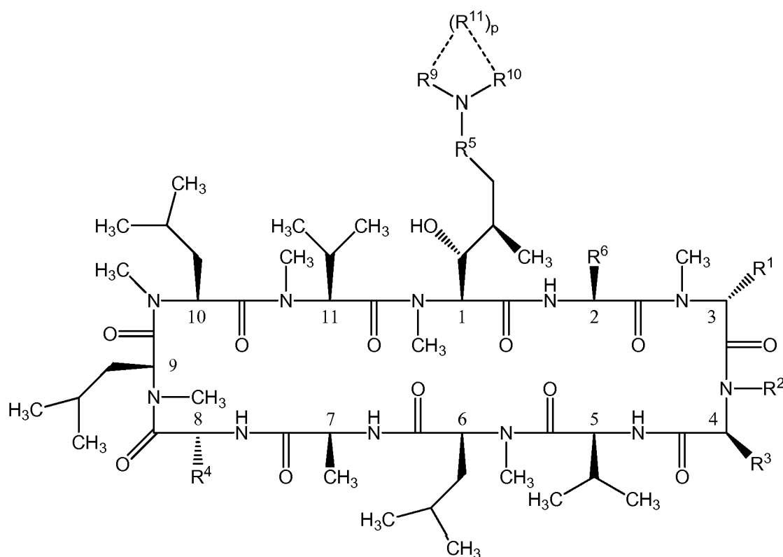
Formula I
