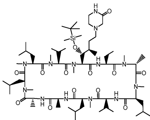
Intermediate 52
