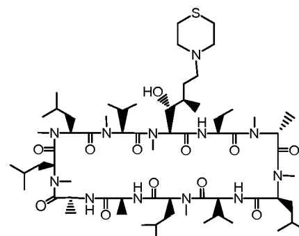
Compound J
