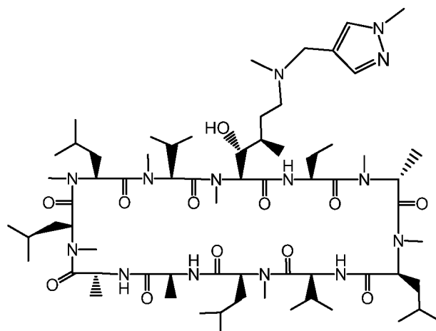
Compound DM
