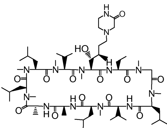
Compound NN
