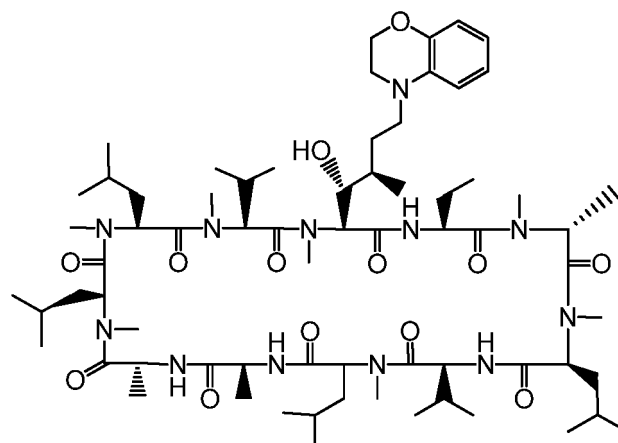
Compound DX
