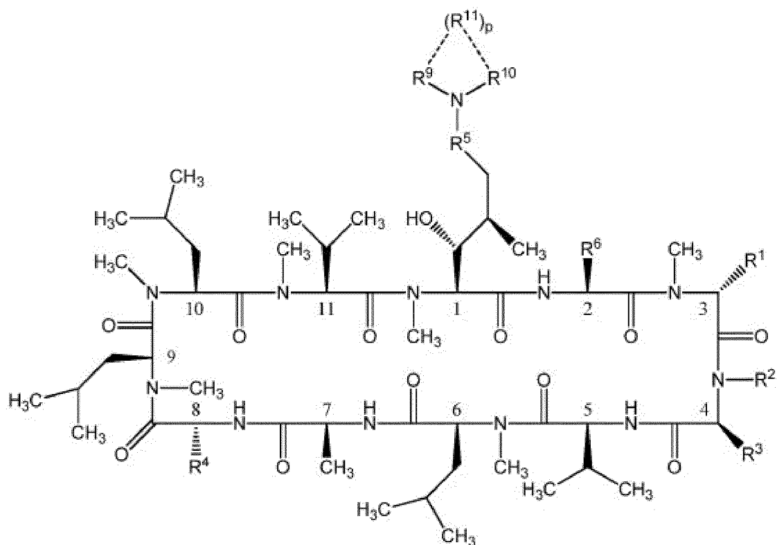
Formel I
