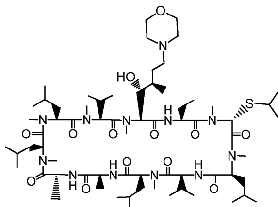
Compound I
