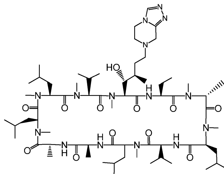
Compound DU
