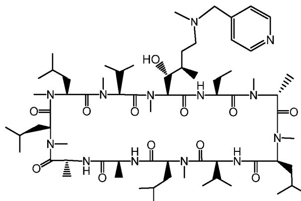
Compound DL
