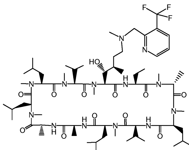
Compound DR
