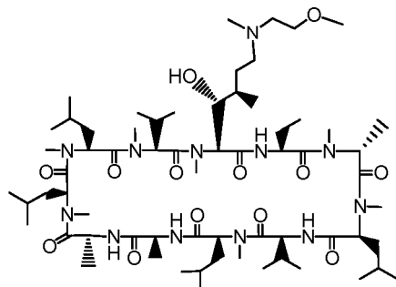
Compound AG
