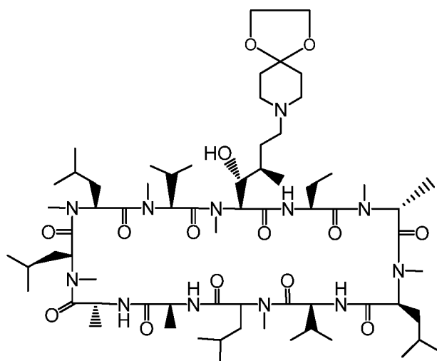
Compound DY
