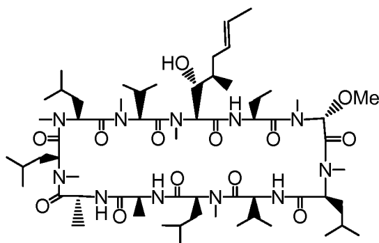
Intermediate 18
