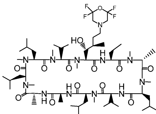
Compound EK
