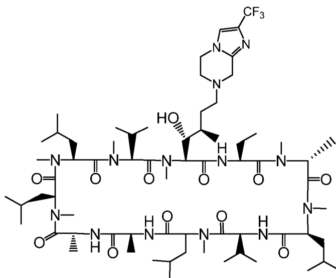
Compound EE
