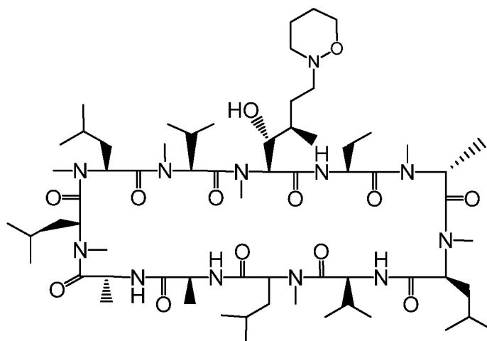
Compound ED
