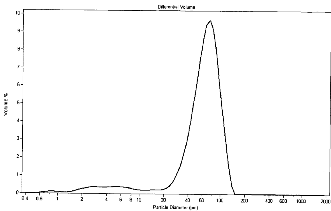
Figure 5: Particle size distribution of the supported catalyst system via Coulter counter
