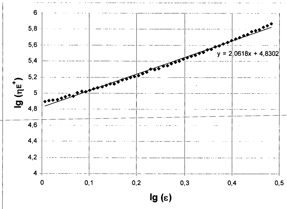
Figure 1: Determination of the SHI of "A" at a strain rate of 0.1\text{s}^{-1} (SHI@ 0.1\text{s}^{-1} )
