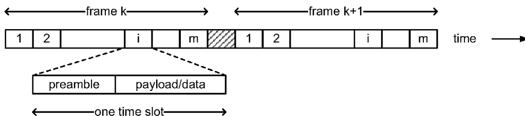
TDMA (Time Division Multiple Access)
