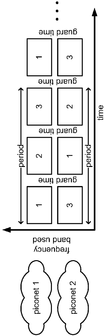
2 synchronized SOPs (Simultaneously Operating Piconets) using TDMA
