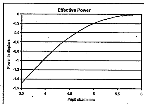
4-Term solution: Effective power over a range of pupil sizes (3.5mm to 6mm)
