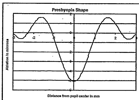
4-Term solution: presbyopia shape
