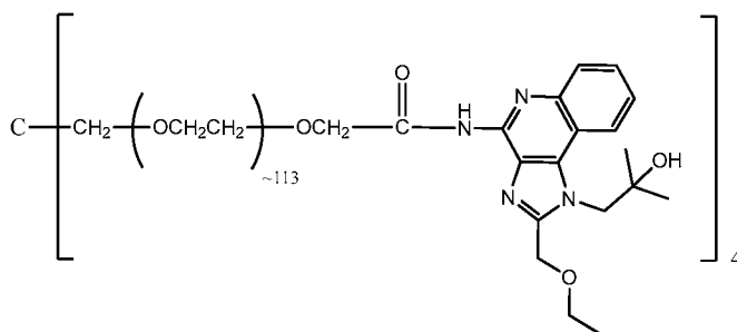
"4-arm-PEG20k-CM-N-R848"
