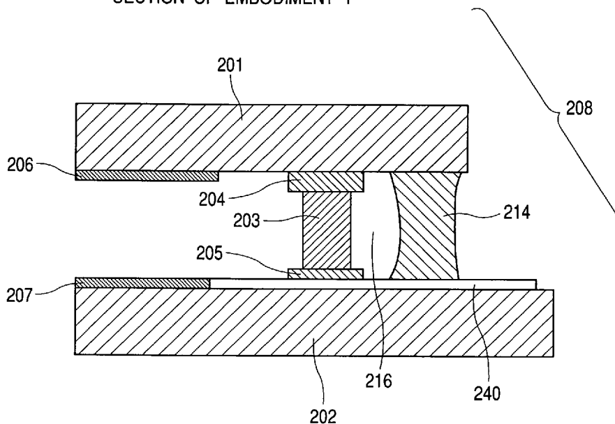
ENLARGED SECTIONAL VIEW OF FRAME SECTION OF EMBODIMENT 1
