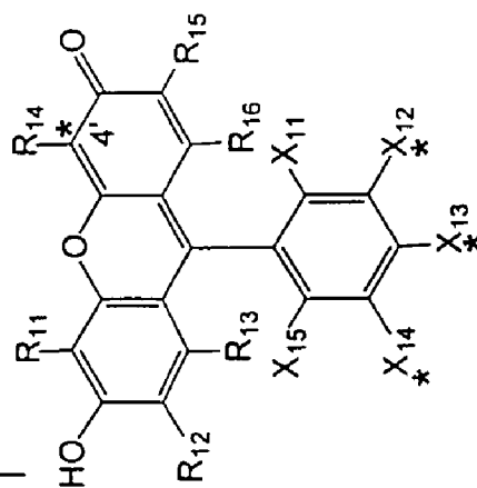
FLUORESCHEIN
