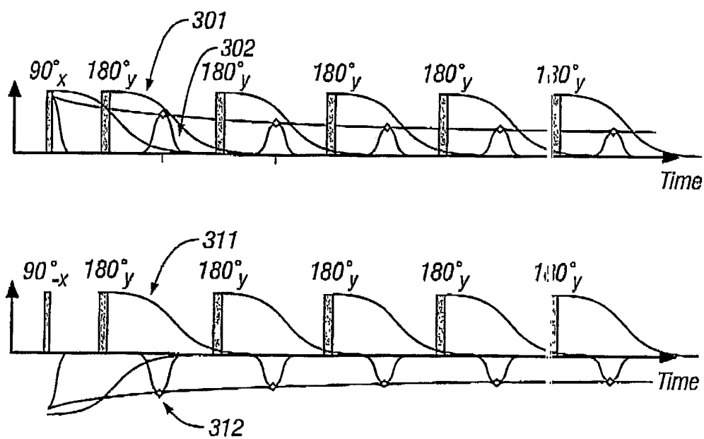
FIG. 3 (Prior Art)
