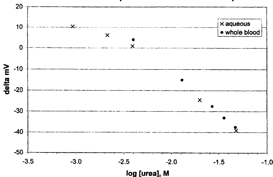
i-STAT BUN sensor response as a function of urea concentration: aqueous and whole blood samples
