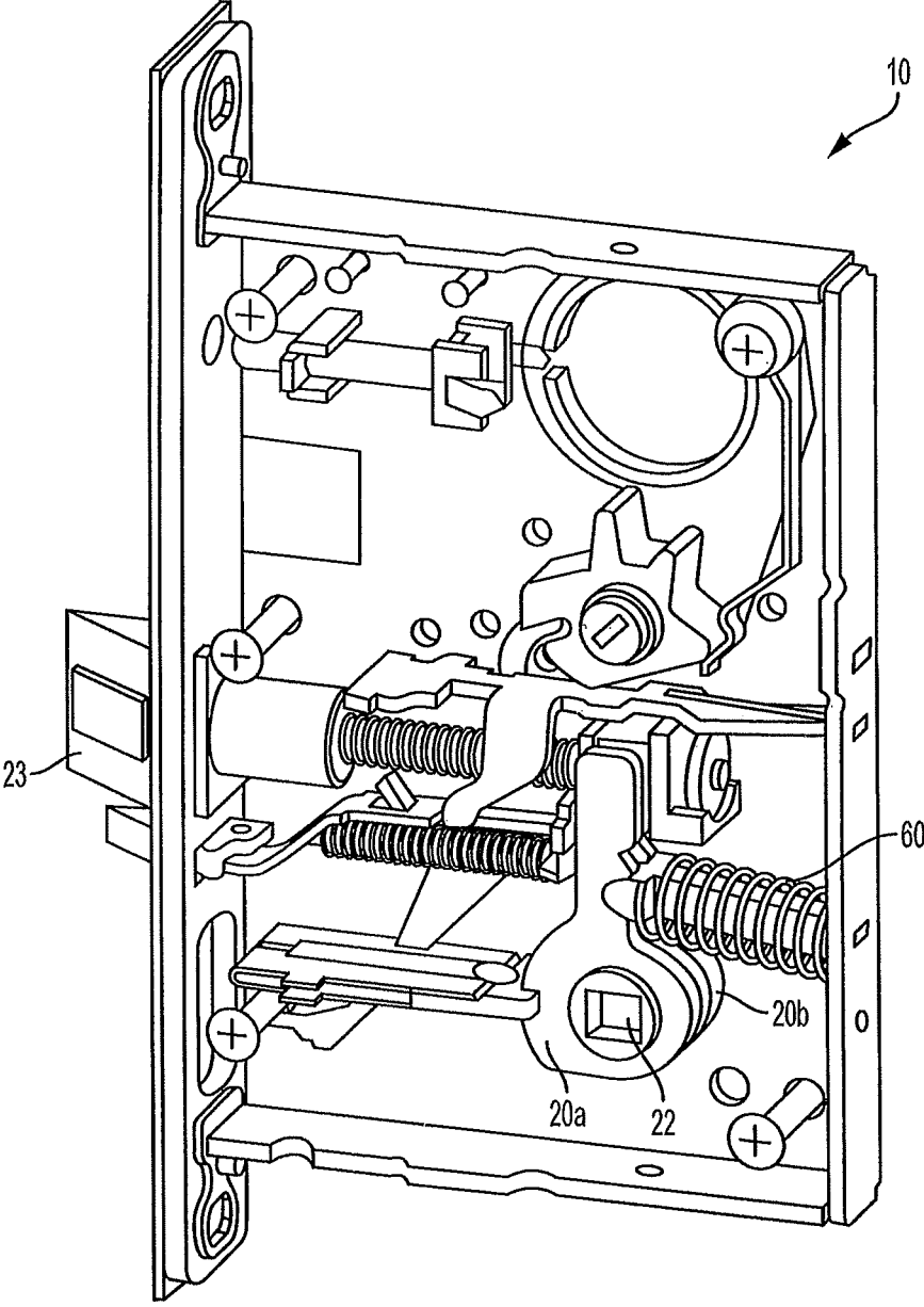
FIG. 3 PRIOR ART
