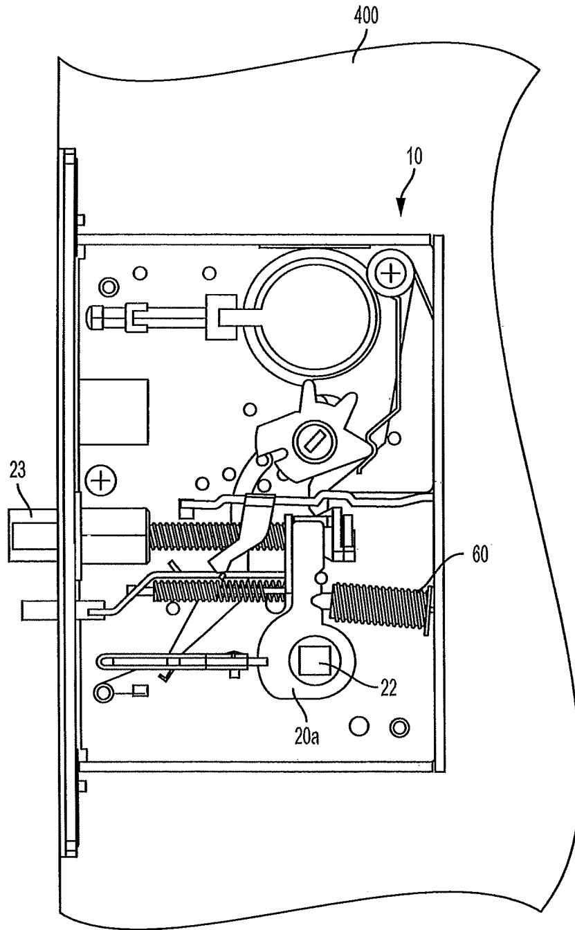
FIG. 2 PRIOR ART
