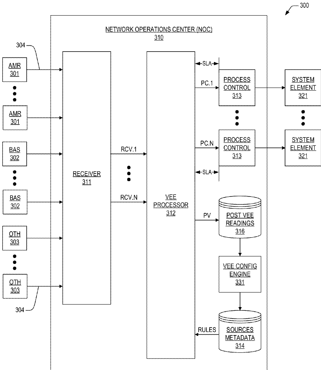
NETWORK OPERATIONS CENTER INCLUDING VEE CONFIGURATION ENGINE
