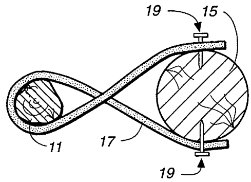
FIG. 2 (PRIOR ART)
