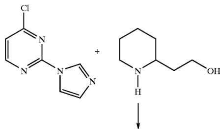
Reaction Scheme 4
