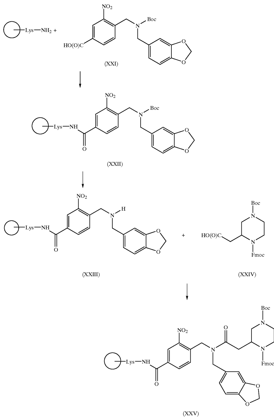
Reaction Scheme 7
