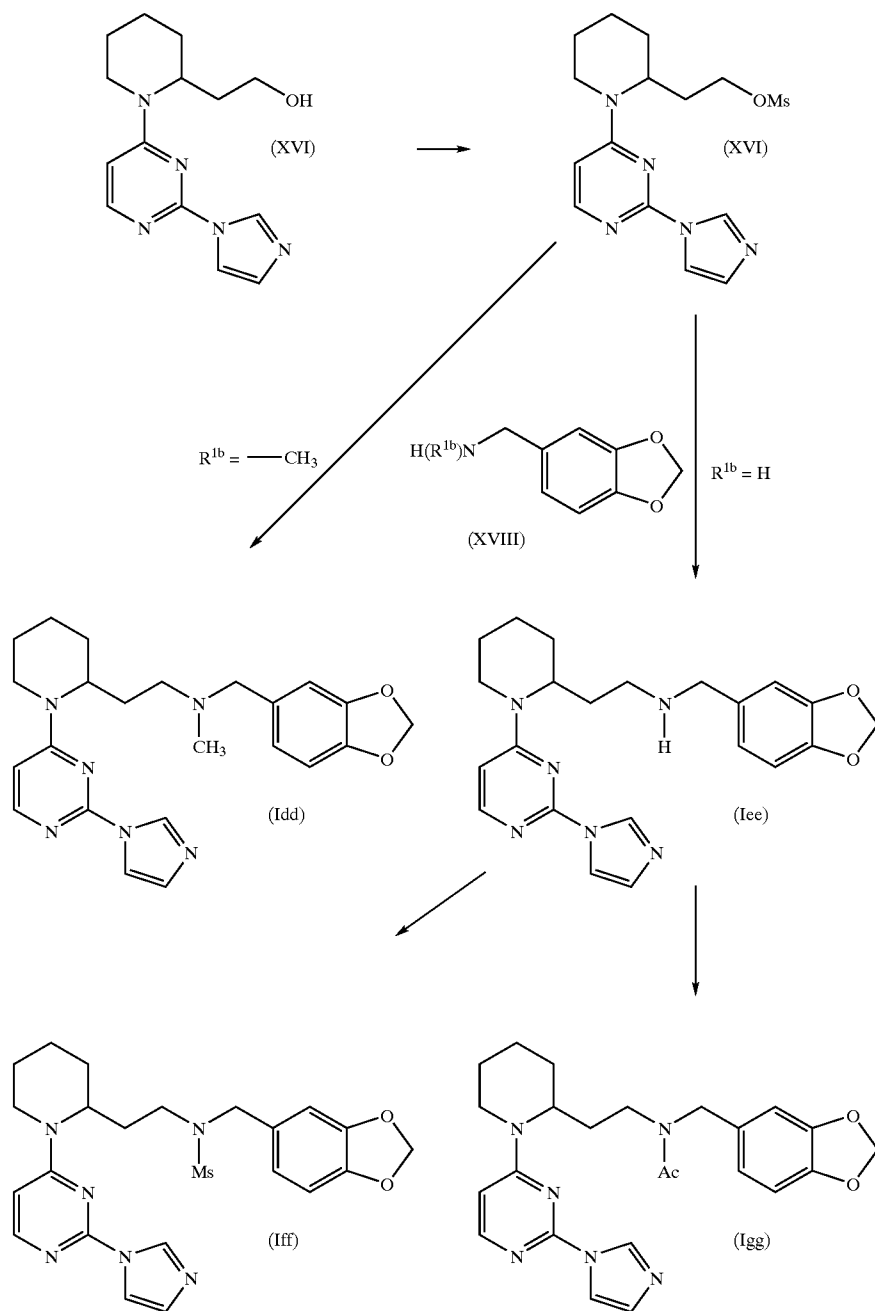
Reaction Scheme 5
