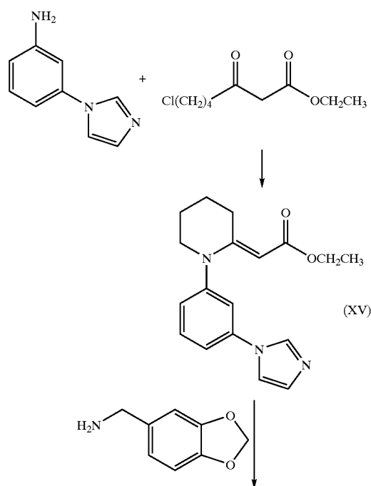
Reaction Scheme 3
