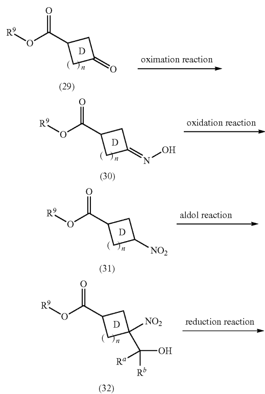
(Scheme 6)
