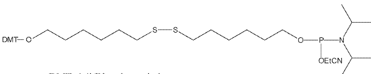
DMT: 4,4'-Dimethoxytrityl
