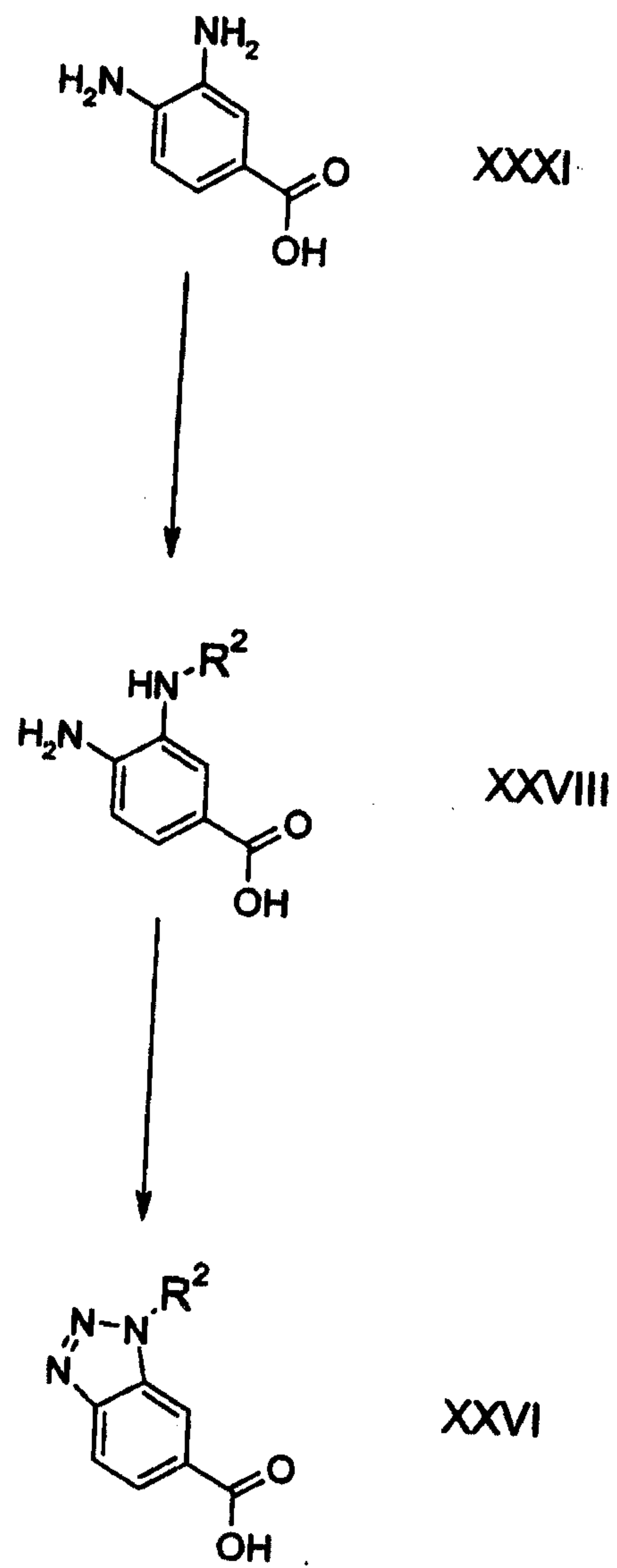
Scheme 8
