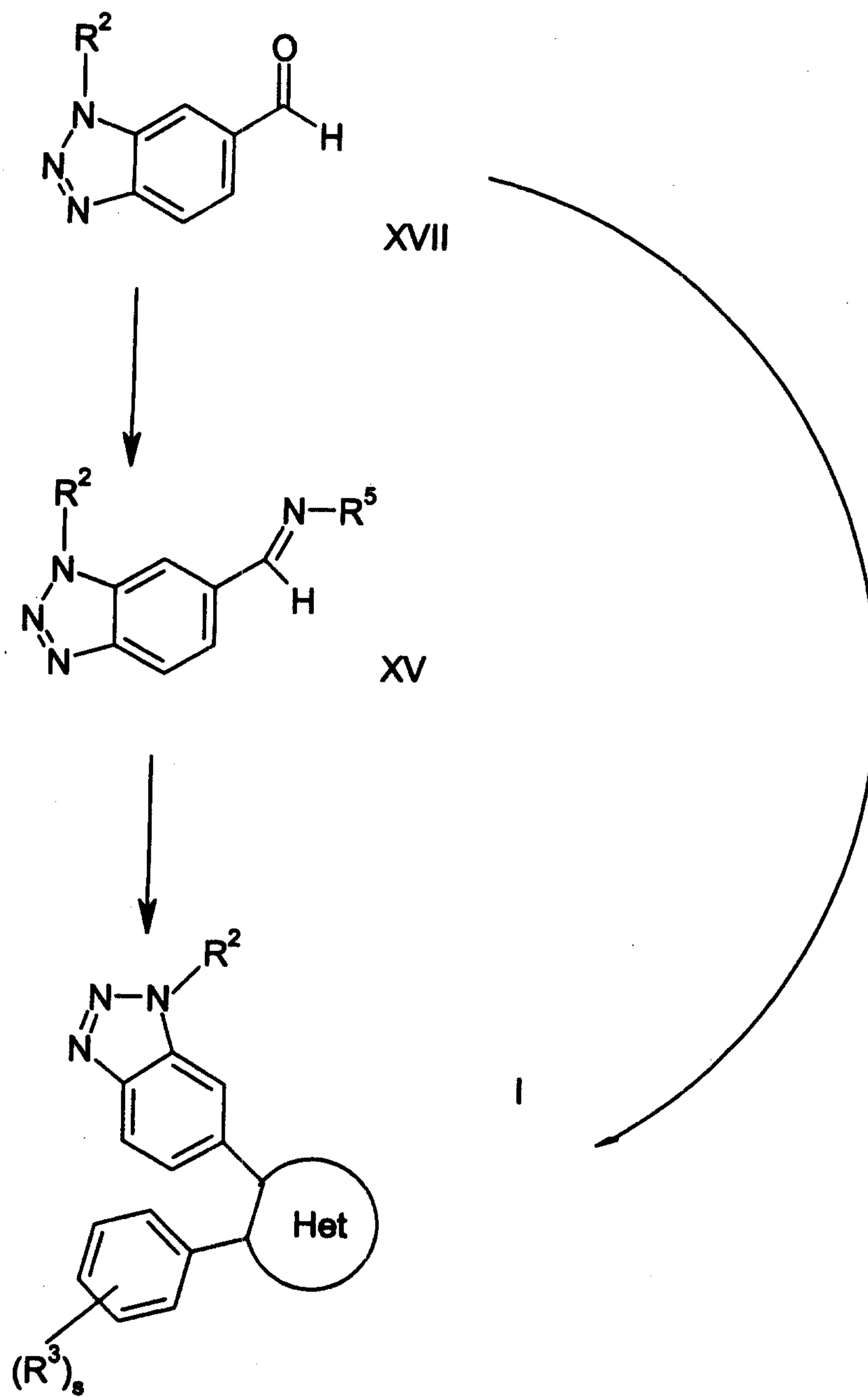
Scheme 3
