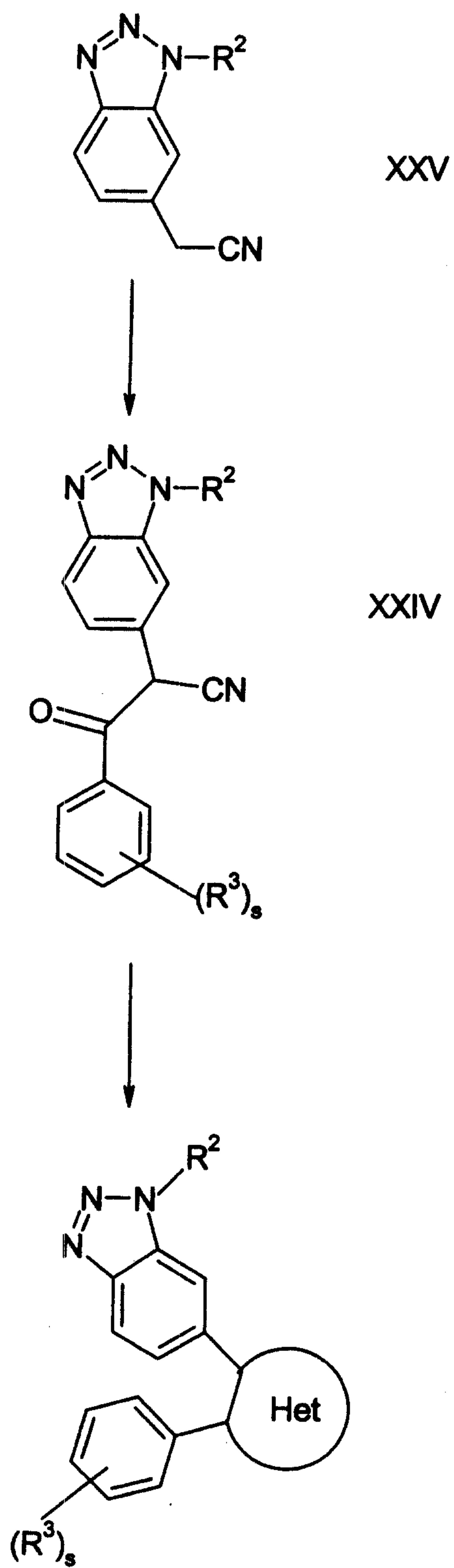
Scheme 5
