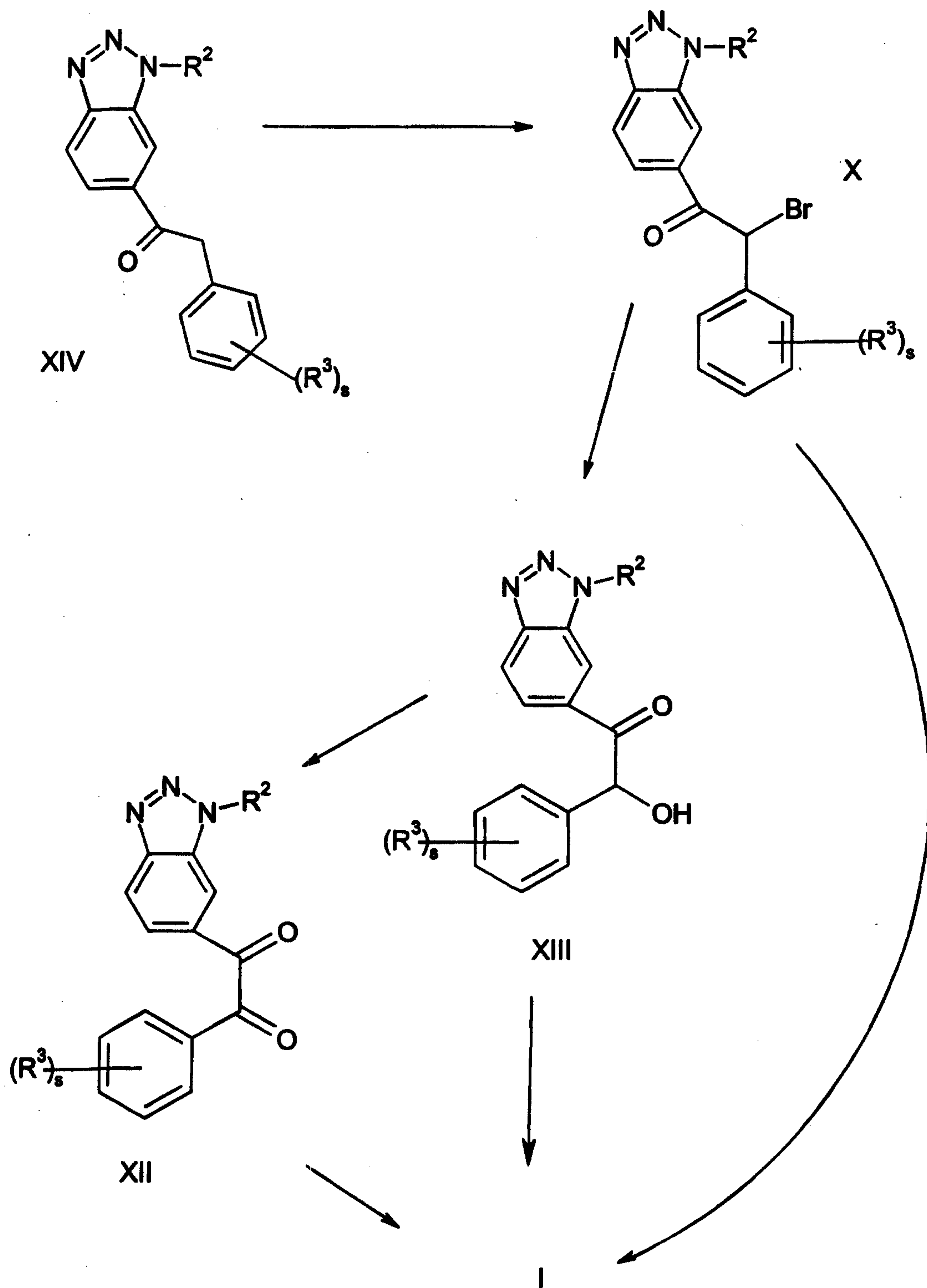
Scheme 2
