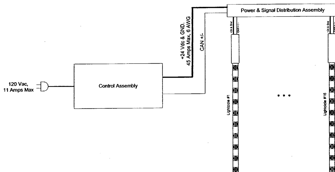
Figure 8 Quadrant System Components and Interconnects
