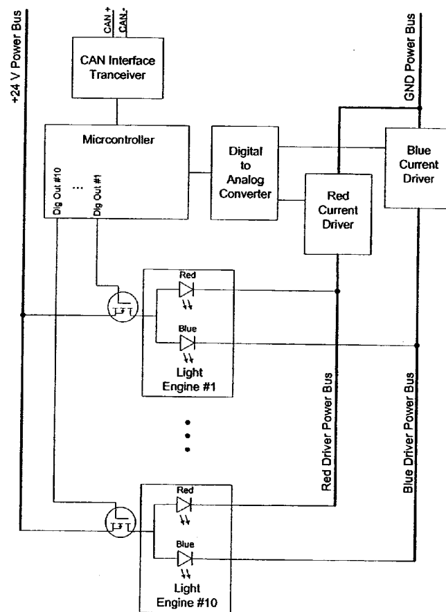
Figure 7 Interface and Driver Electronics Block Diagram
