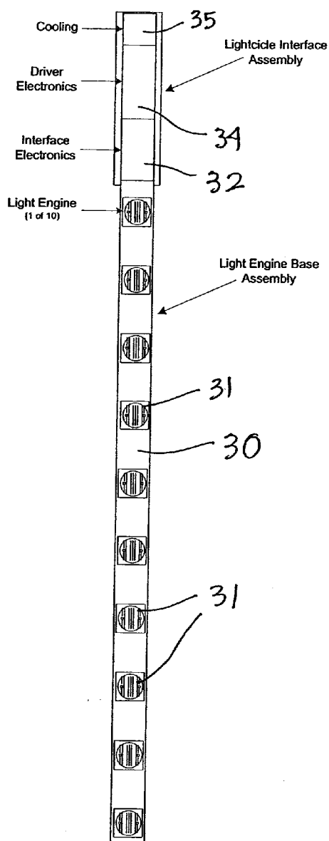
Figure 6 Lightcicle Basic Structure
