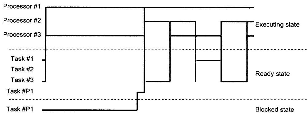
Figure 27: Three processor 3 timeslice tasks, 1 pre-emption task
