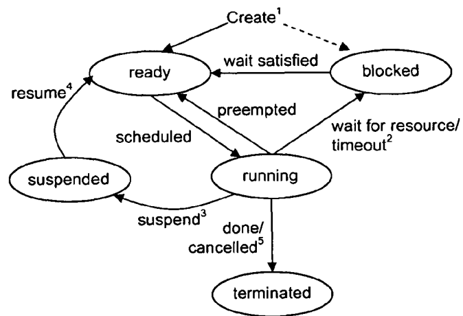
Figure 1: Task state diagram
