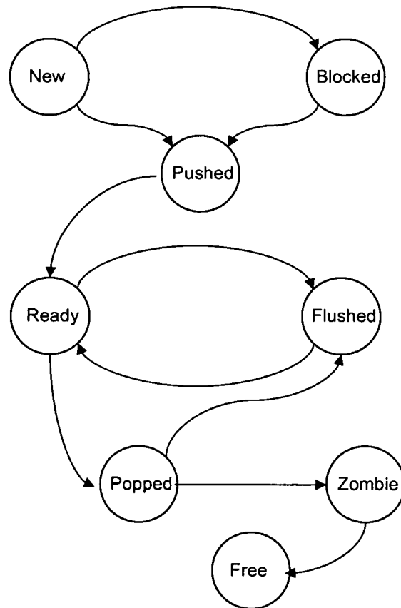
Figure 41: SystemWeaver internal thread state diagram
