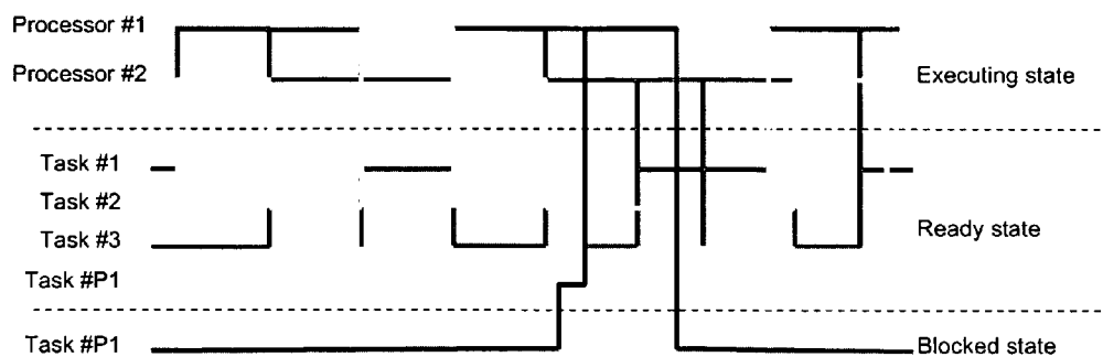
Figure 26: Dual processor 3 timeslice tasks, 1 pre-emption task
