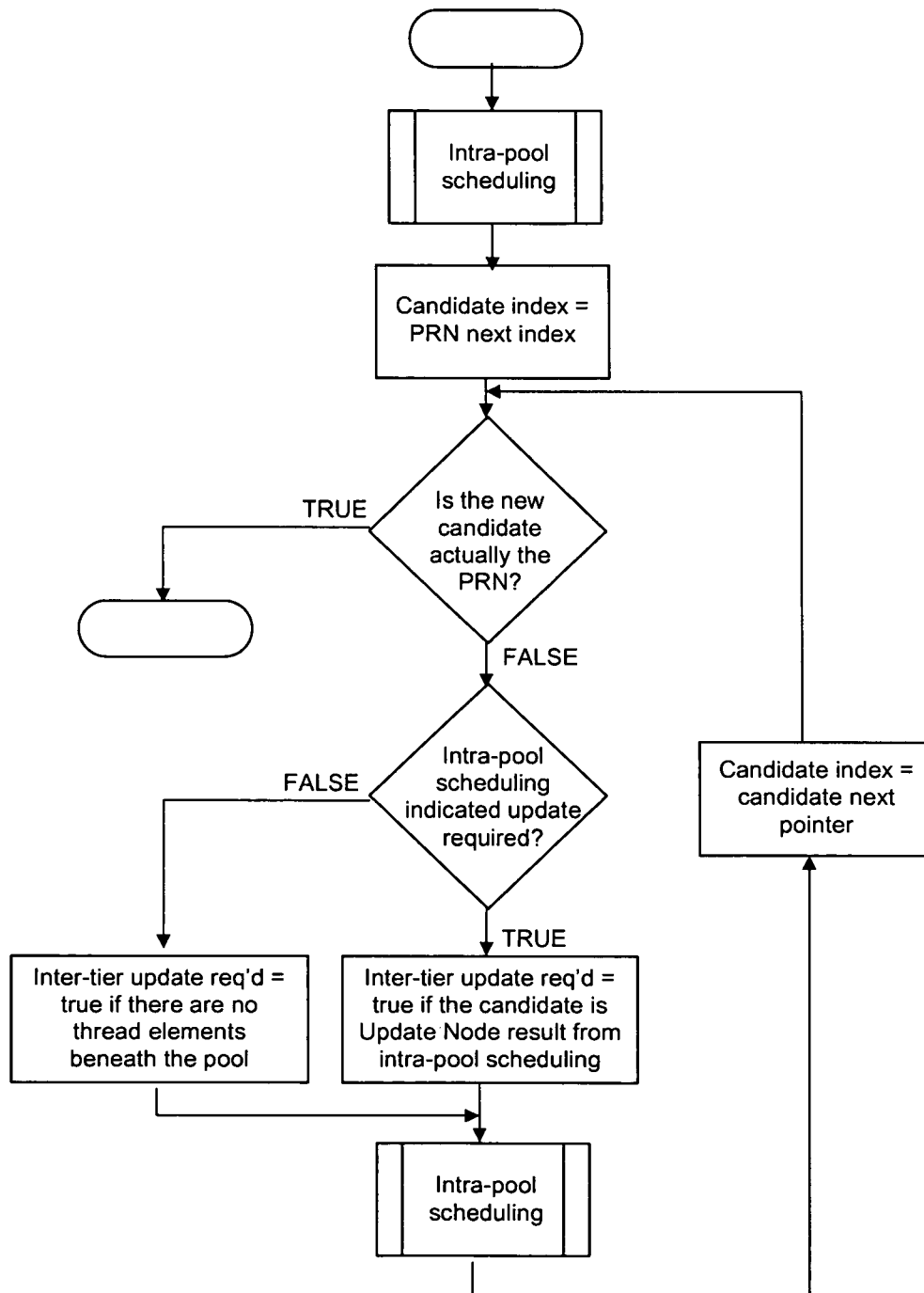
Figure 66: Inter-pool distribution tier scheduler processing
