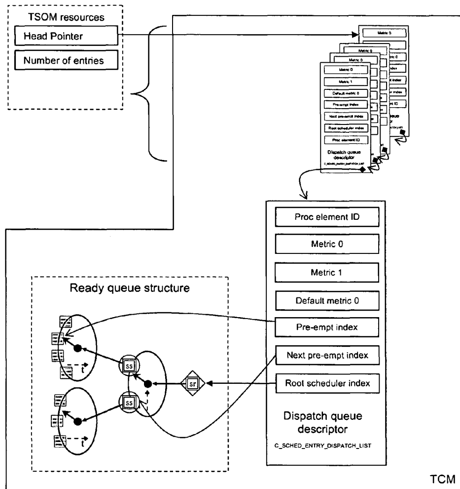
Figure 58: TSOM internal architecture
