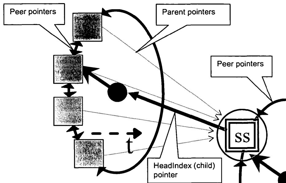
Figure 12: Scheduling tier pointer configuration
