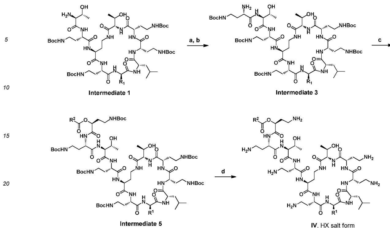
Scheme 3. General synthesis of the compounds of formula IV where p is 1.
