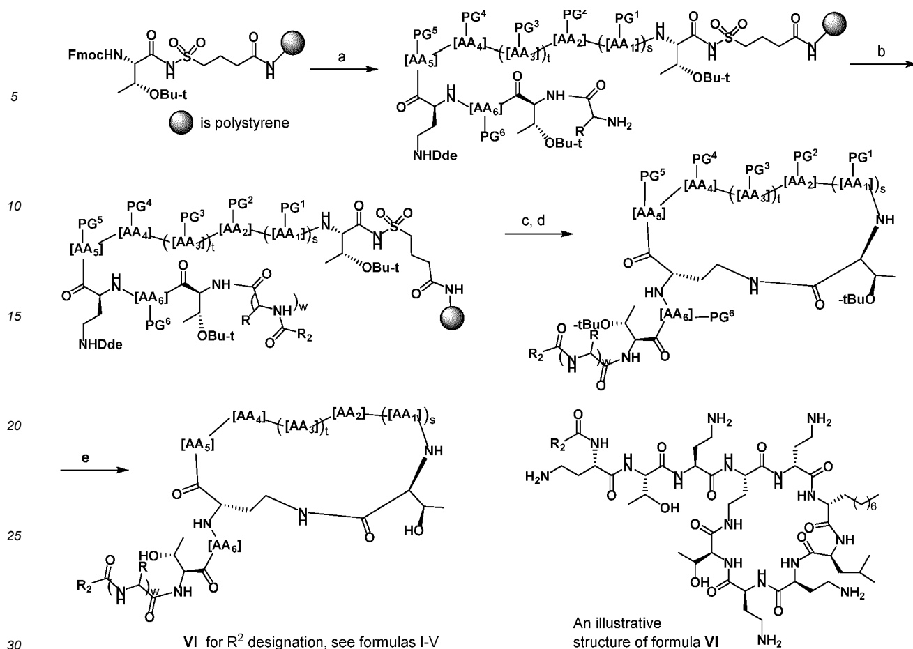
Scheme 5. General synthesis of compounds of formula VI analogous to those of formulas I-V incorporating various amino acids optionally replacing those in formulas I-V.
