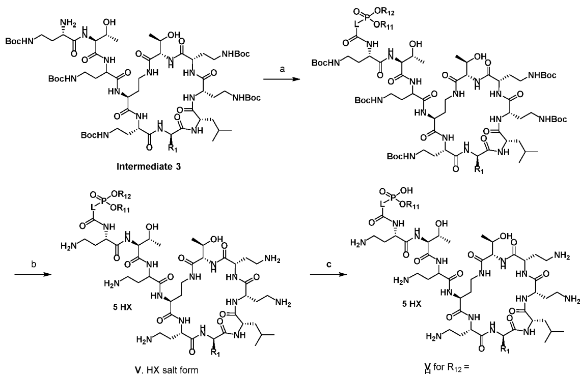
Scheme 4. General synthesis of the compounds of formula V where p is 1.
