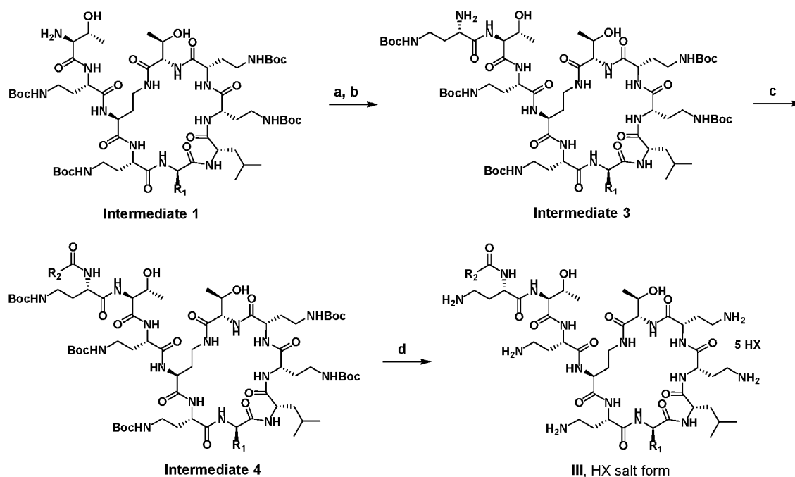
Scheme 2. General synthesis of the compounds of formula III where p is 1.
