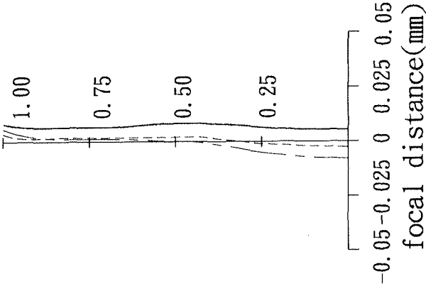
longitudinal spherical aberration
